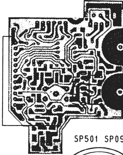
B551 PA-245 LED PCB (TOP VIEW)
