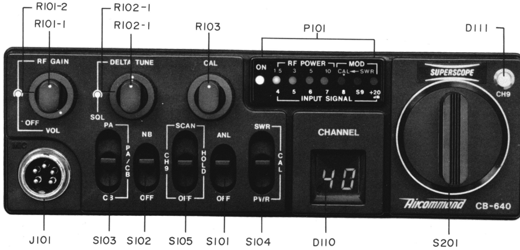
Figure 6 Front View.
