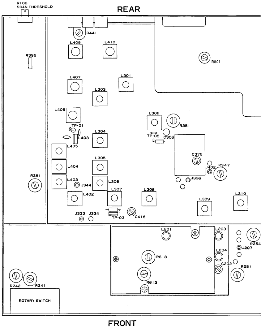
Figure 10 Adjusting and Test Points on Upper Side.
