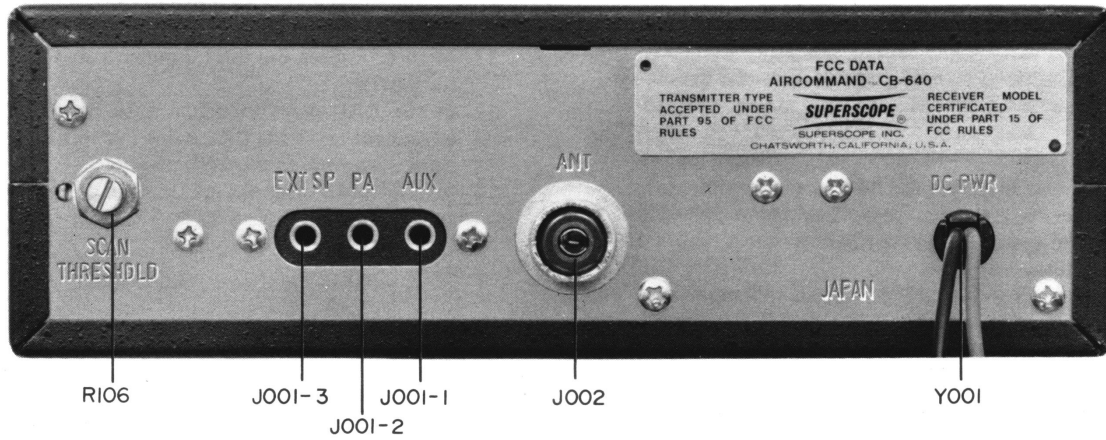
Figure 7 Rear View.
