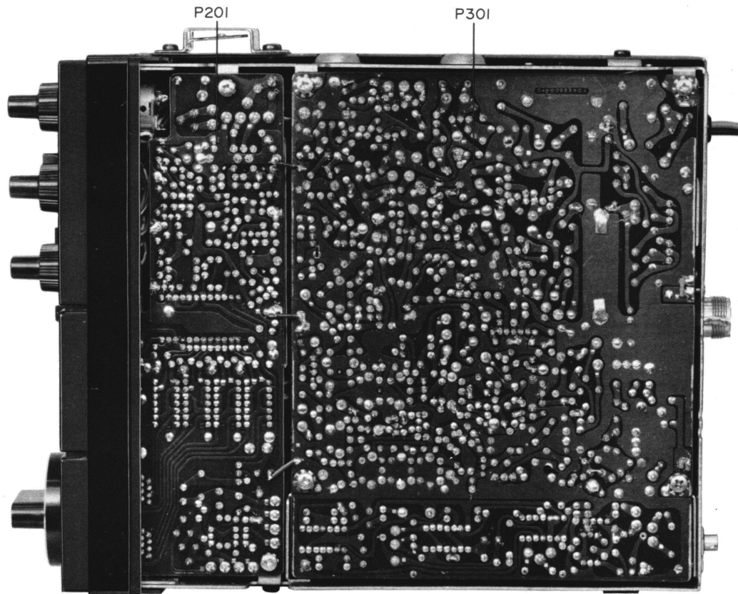
Figure 9 Inside Bottom View.
