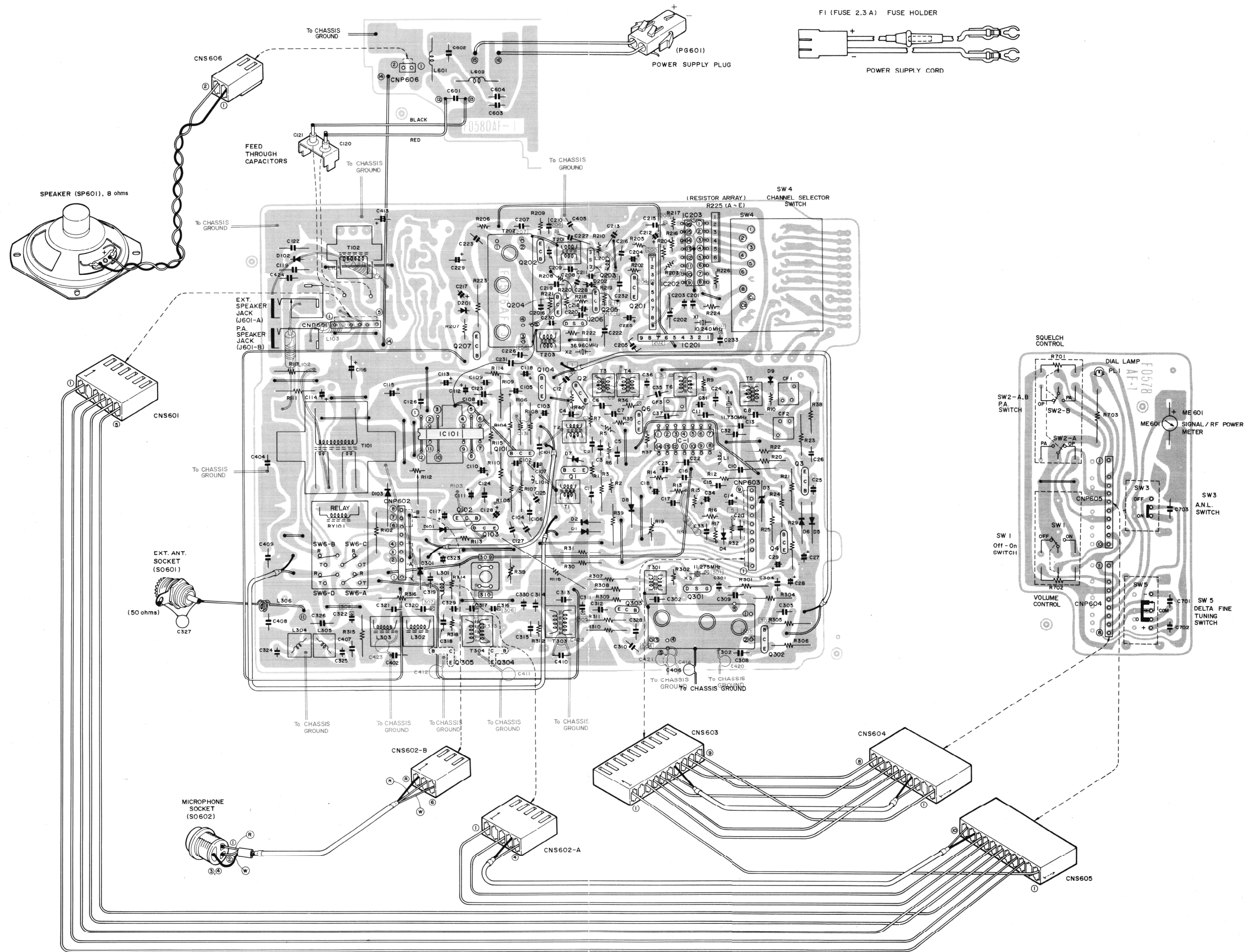
Figure 10 WIRING SIDE OF P.W. BOARD
