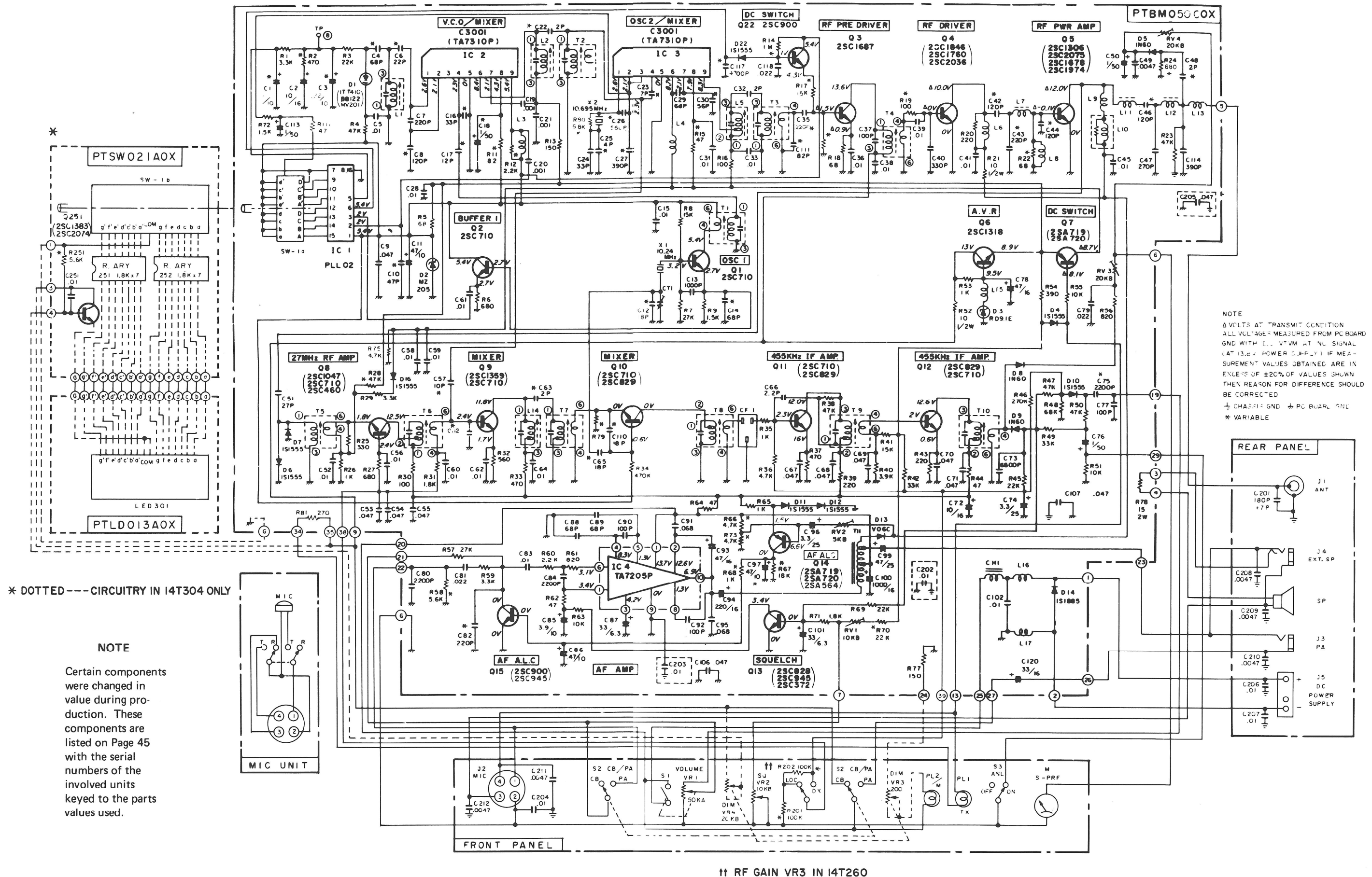
Figure 34 - Schematic Diagram of 14T260 & 14T304
