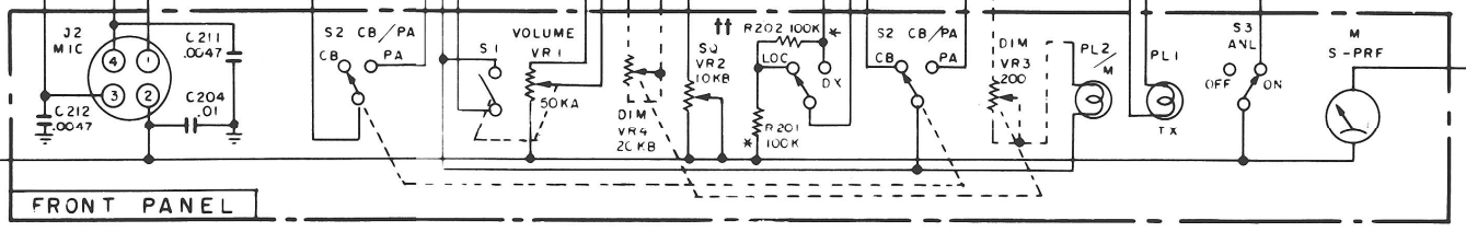
Figure 34 - Schematic Diagram of 14T260 & 14T304
