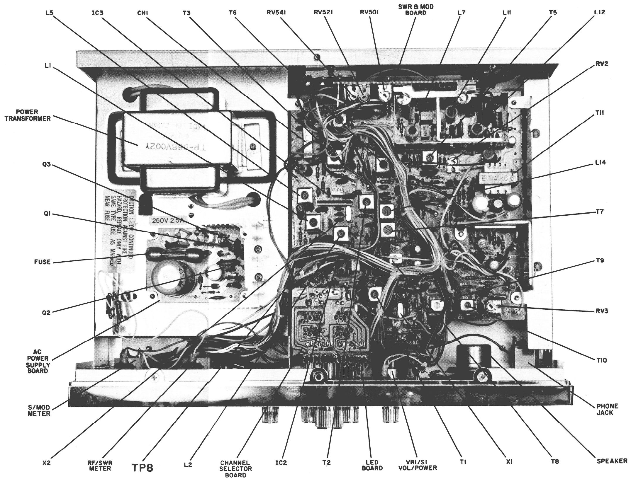
Figure 18 – Top (Component) View of Model 14T303
