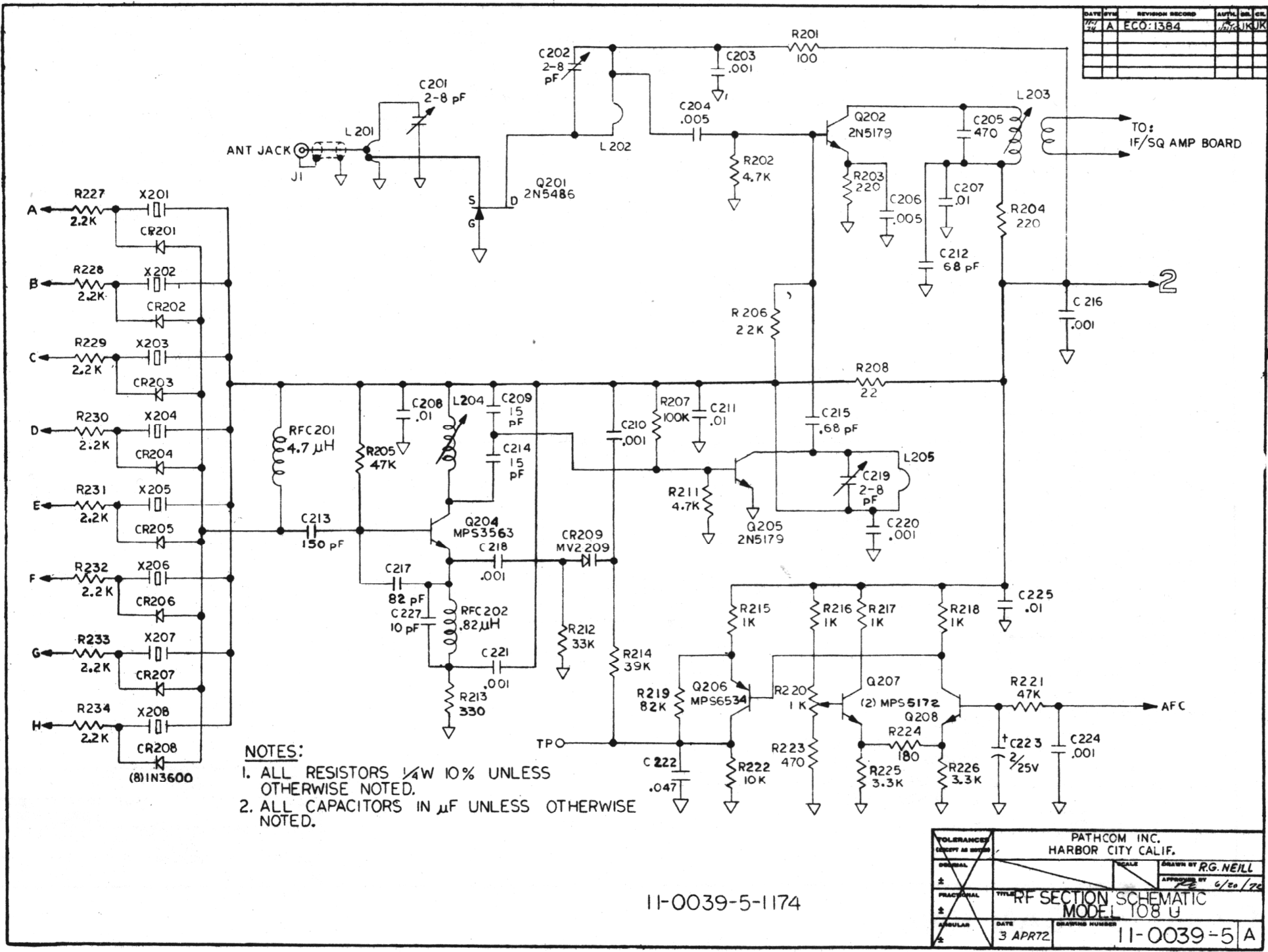
Figure 6-13. UHF/RF Circuit for SCAN 108U
