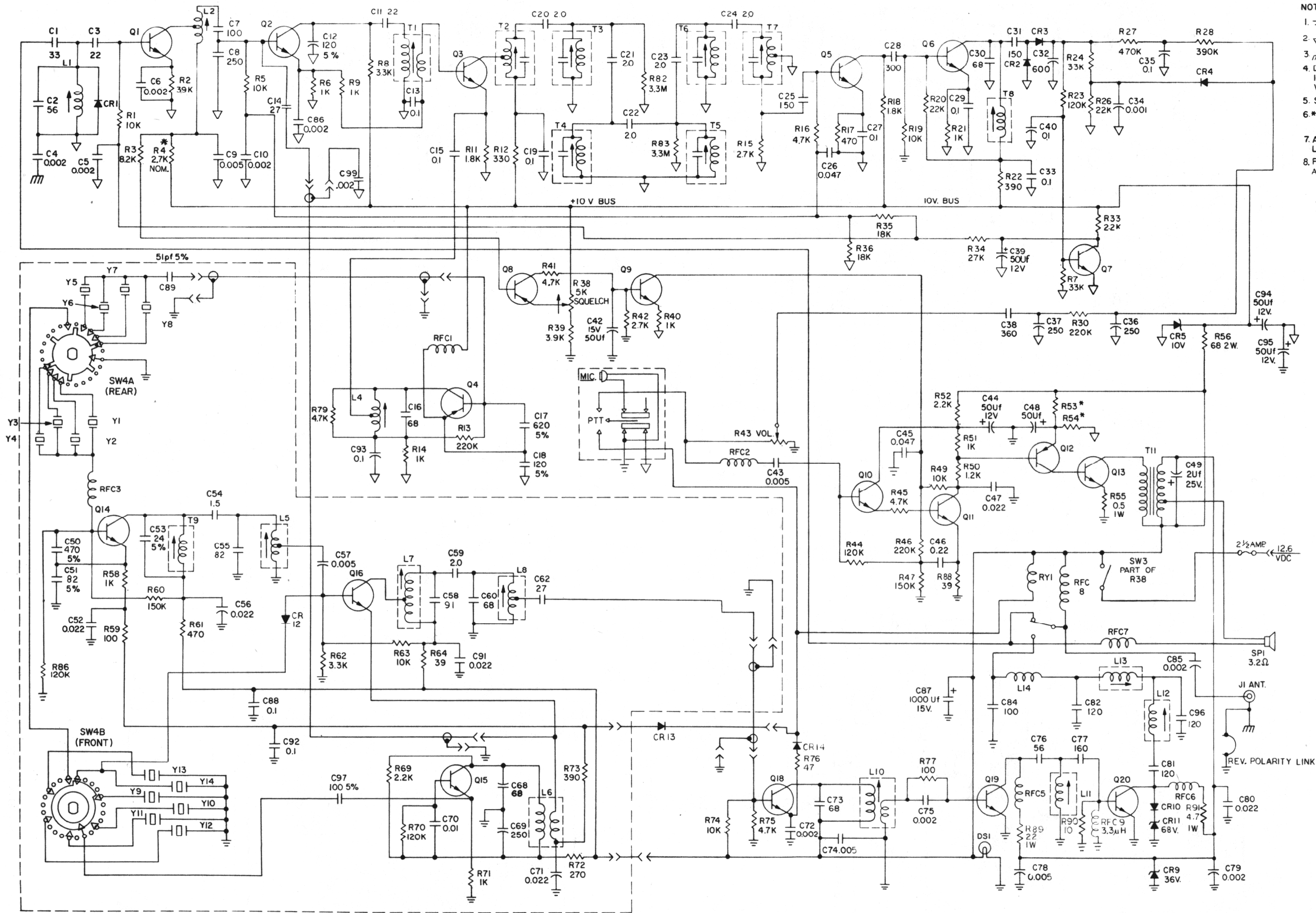
SCHEMATIC DIAGRAM MODEL 223 PATHCOM INC. 11-0036 D REDRAWN BY JK
