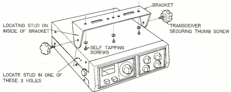
FIGURE 3 Transceiver Mounting
