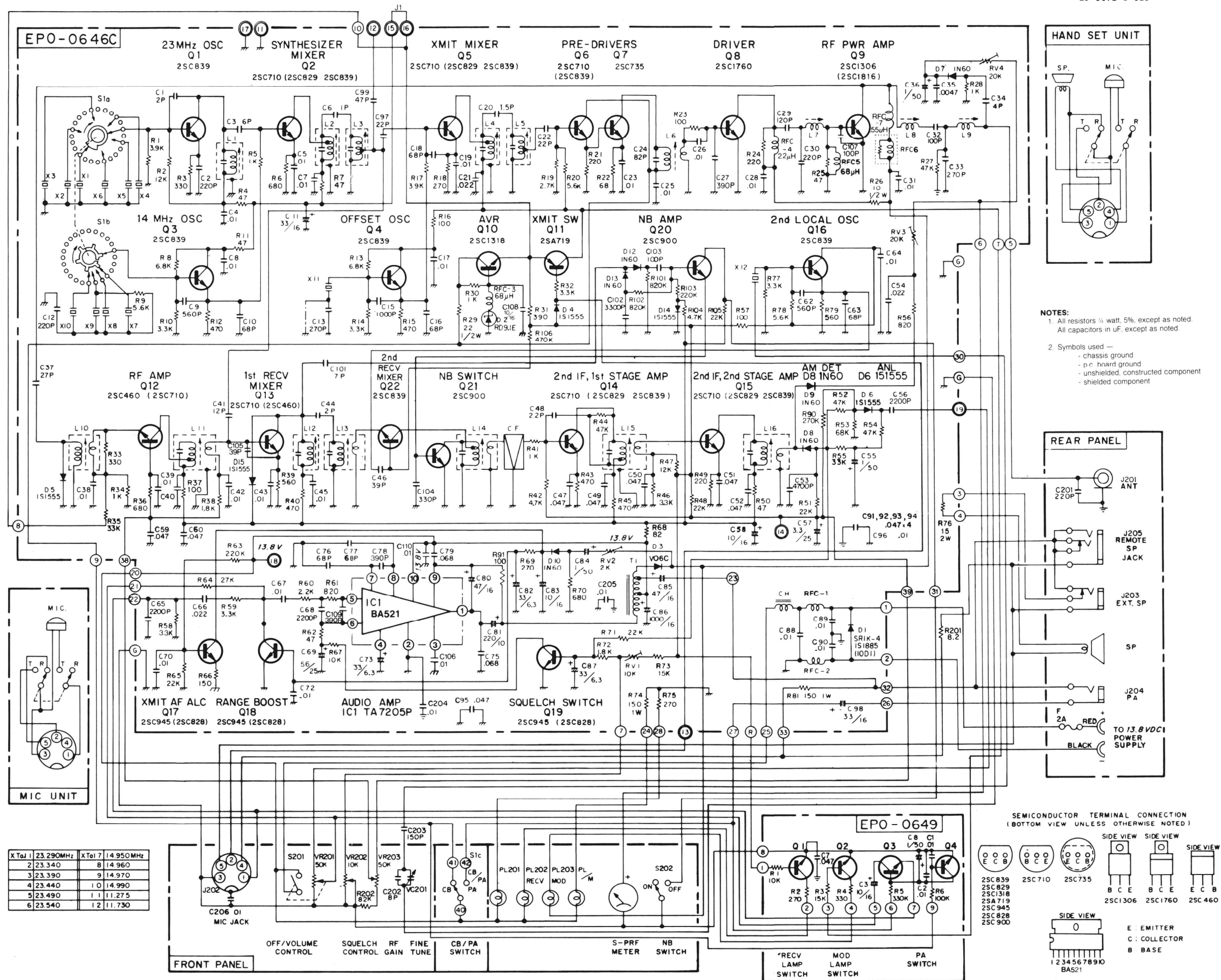
Figure 4-9. Schematic Diagram, 6/25, Stage 4
