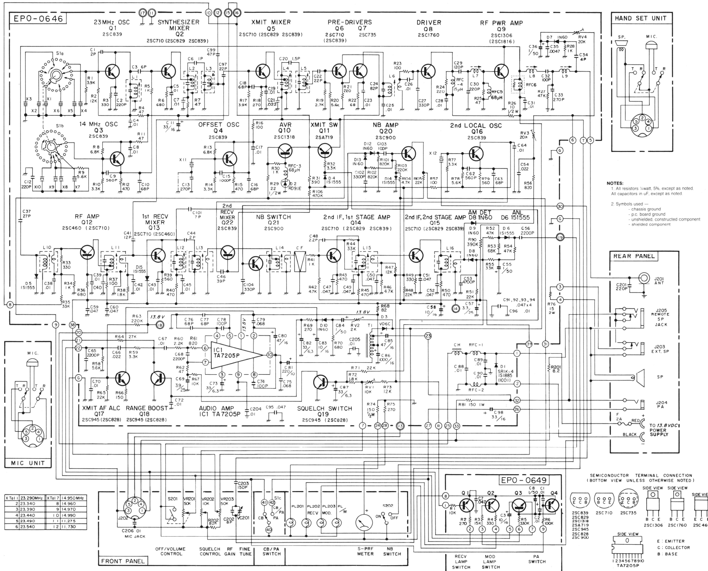
Figure 4-6. Schematic Diagram, 672B, Stage 1
