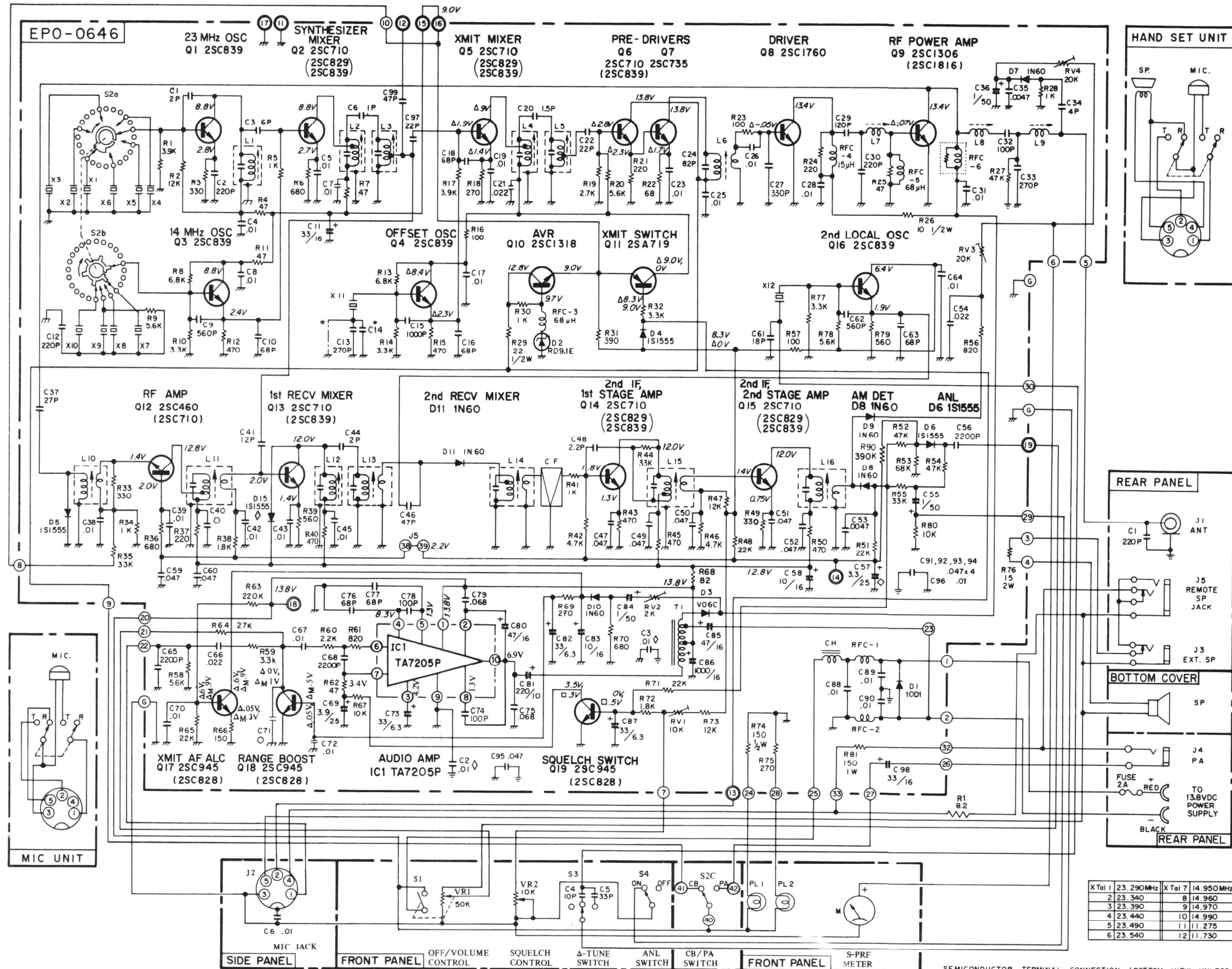
Figure 4-8. Schematic Diagram, 671B, Stage 1
