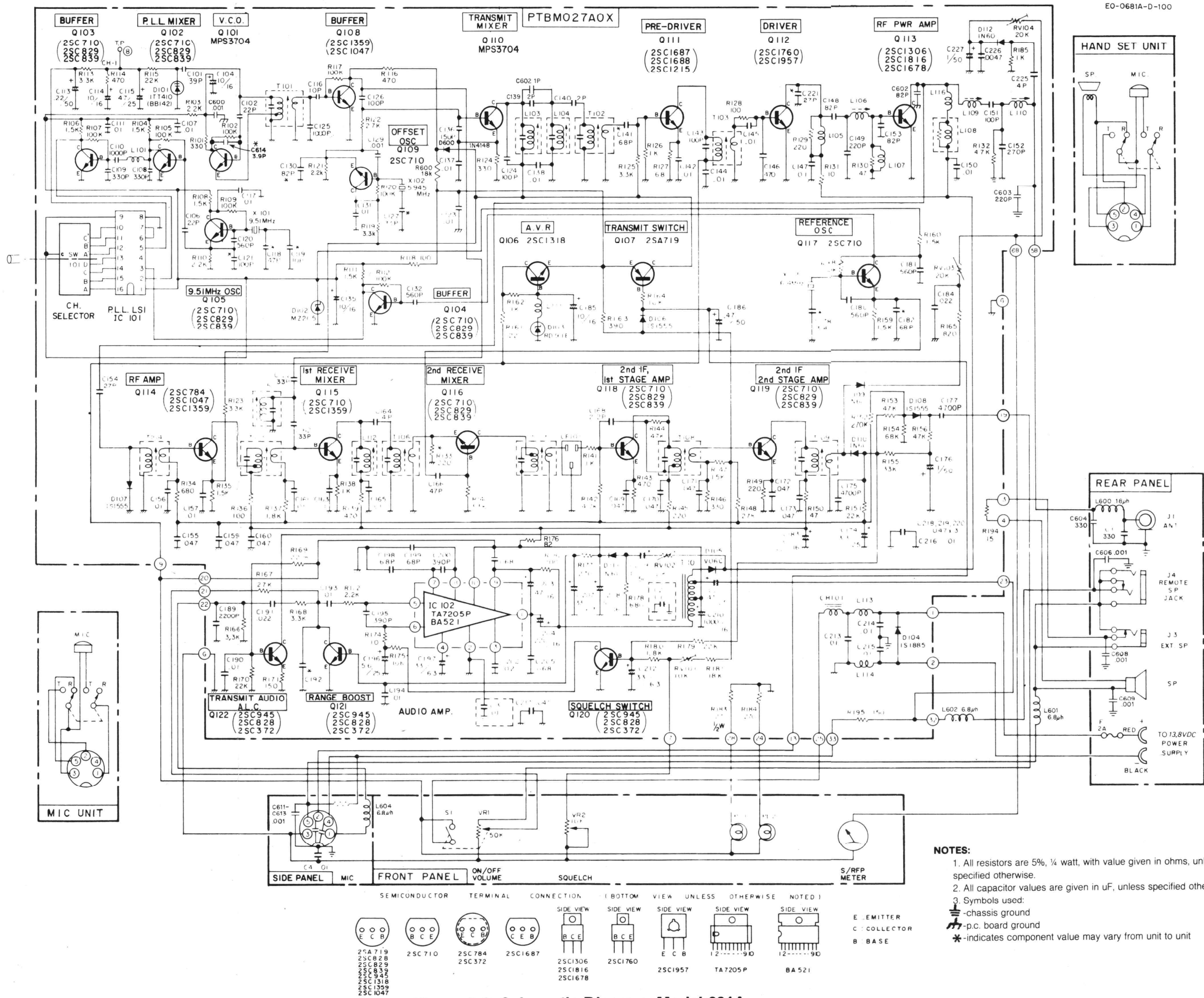
Figure 4-6. Schematic Diagram, Model 681A
