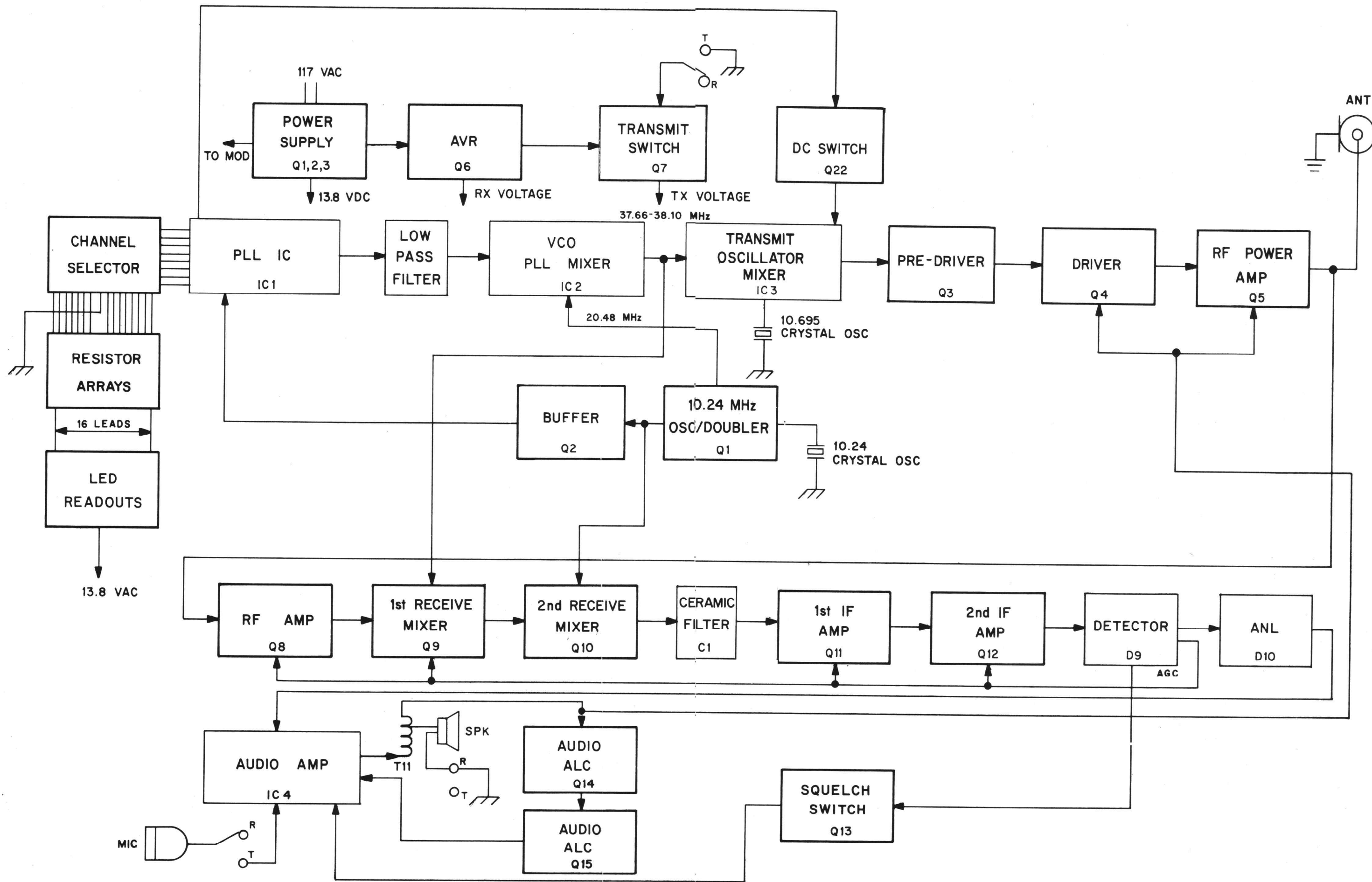
Figure 2-2. Block Diagram, Model 3107
