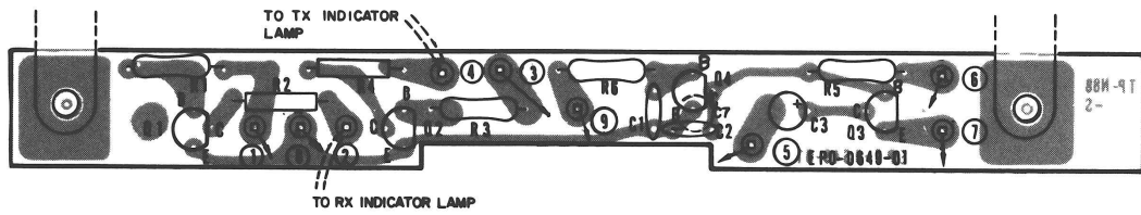
Figure 4-4. Front Panel Lamp Controller P.C. Board Component Outline (2683 Only)
