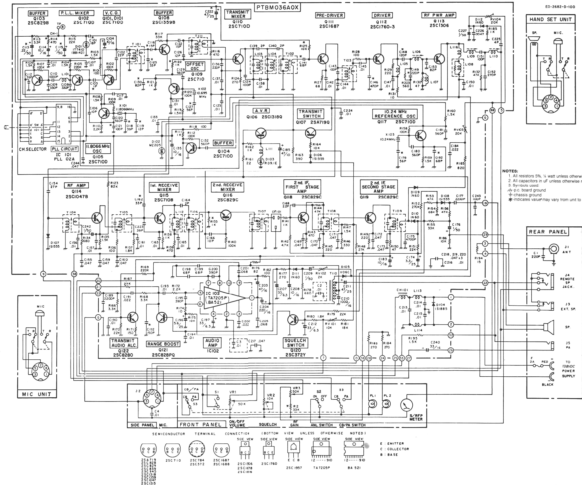
Figure 4-7 Schematic Diagram, Model 2682
