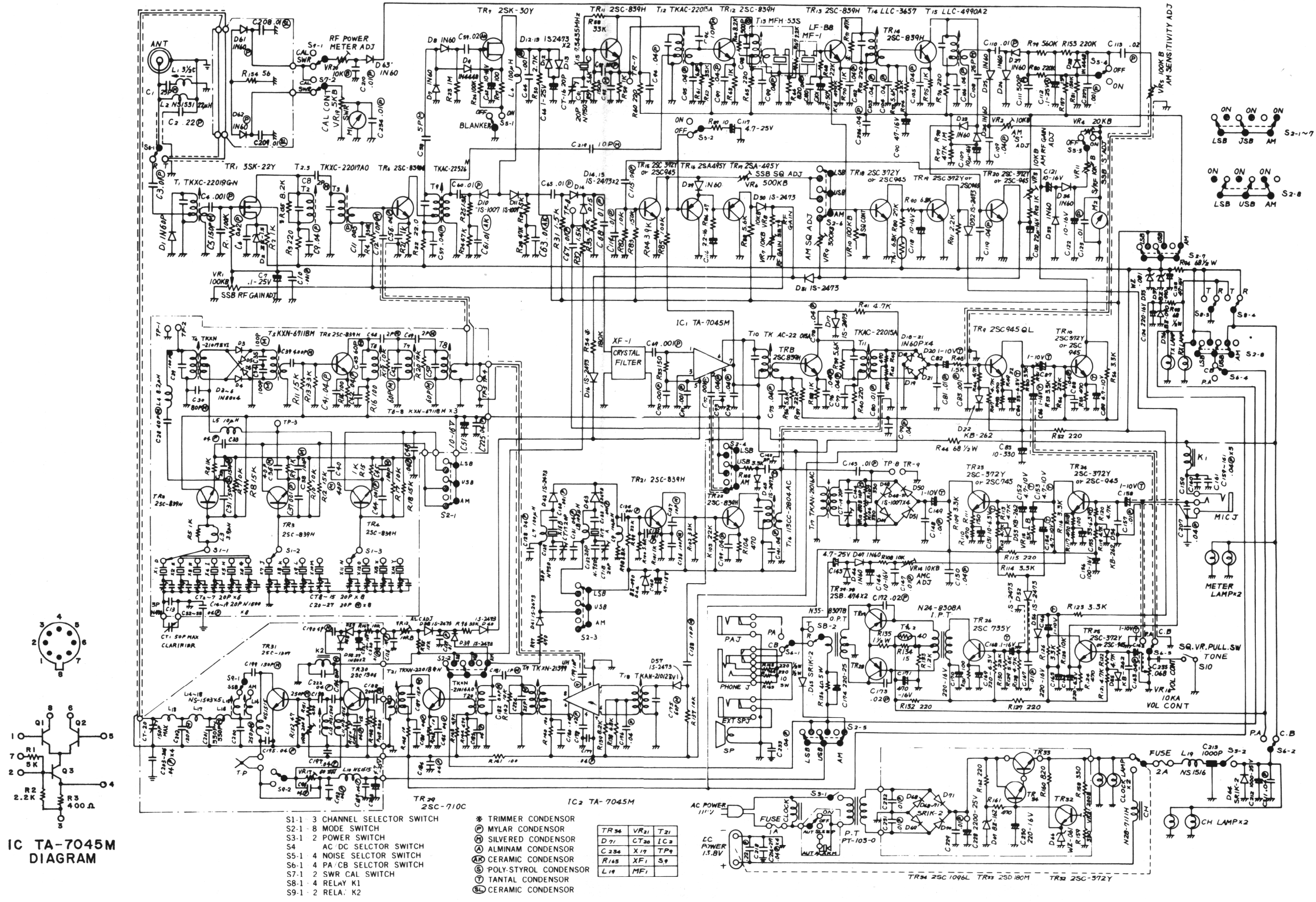
FIGURE 12, SCHEMATIC DIAGRAM
