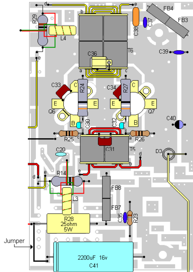
Board C Top View Used up till about 5 years ago
