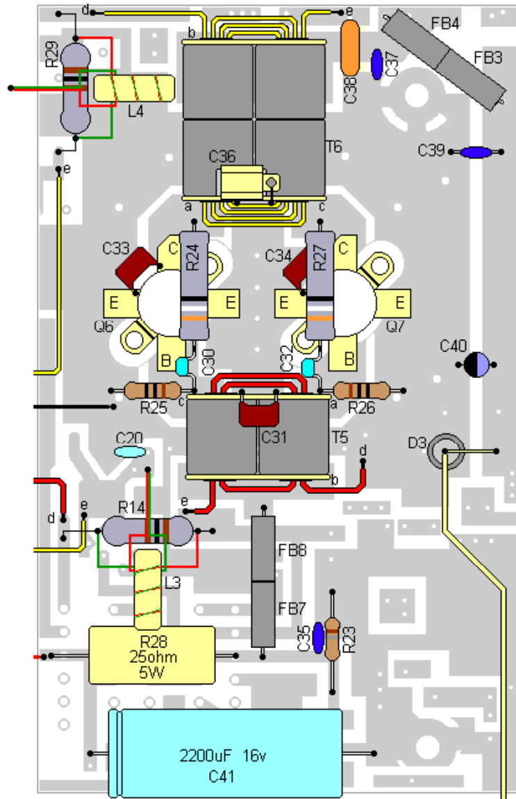
Board D Top View Current Production
