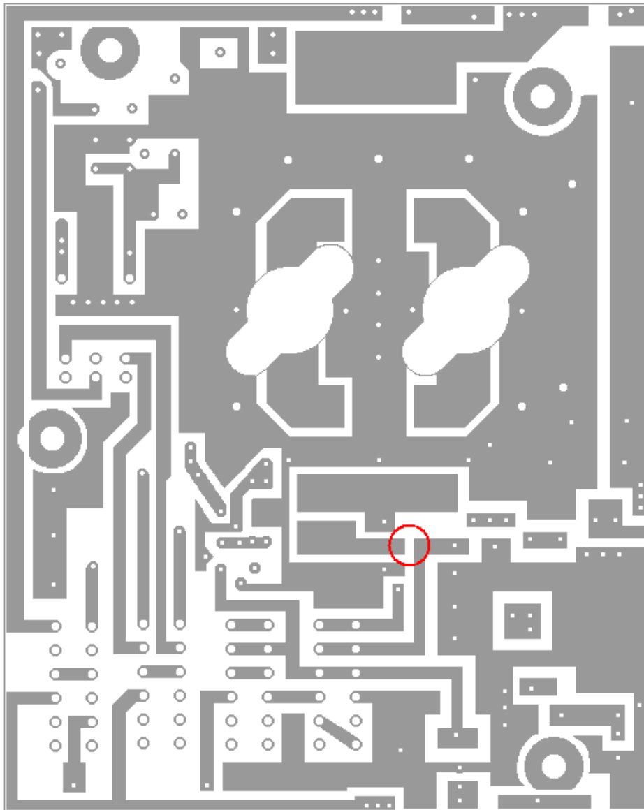
Board Top View
