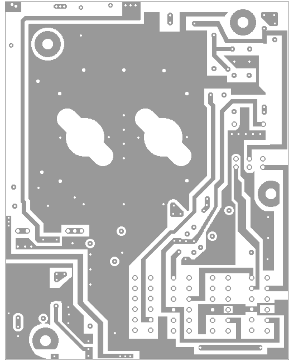
Board Bottom View
