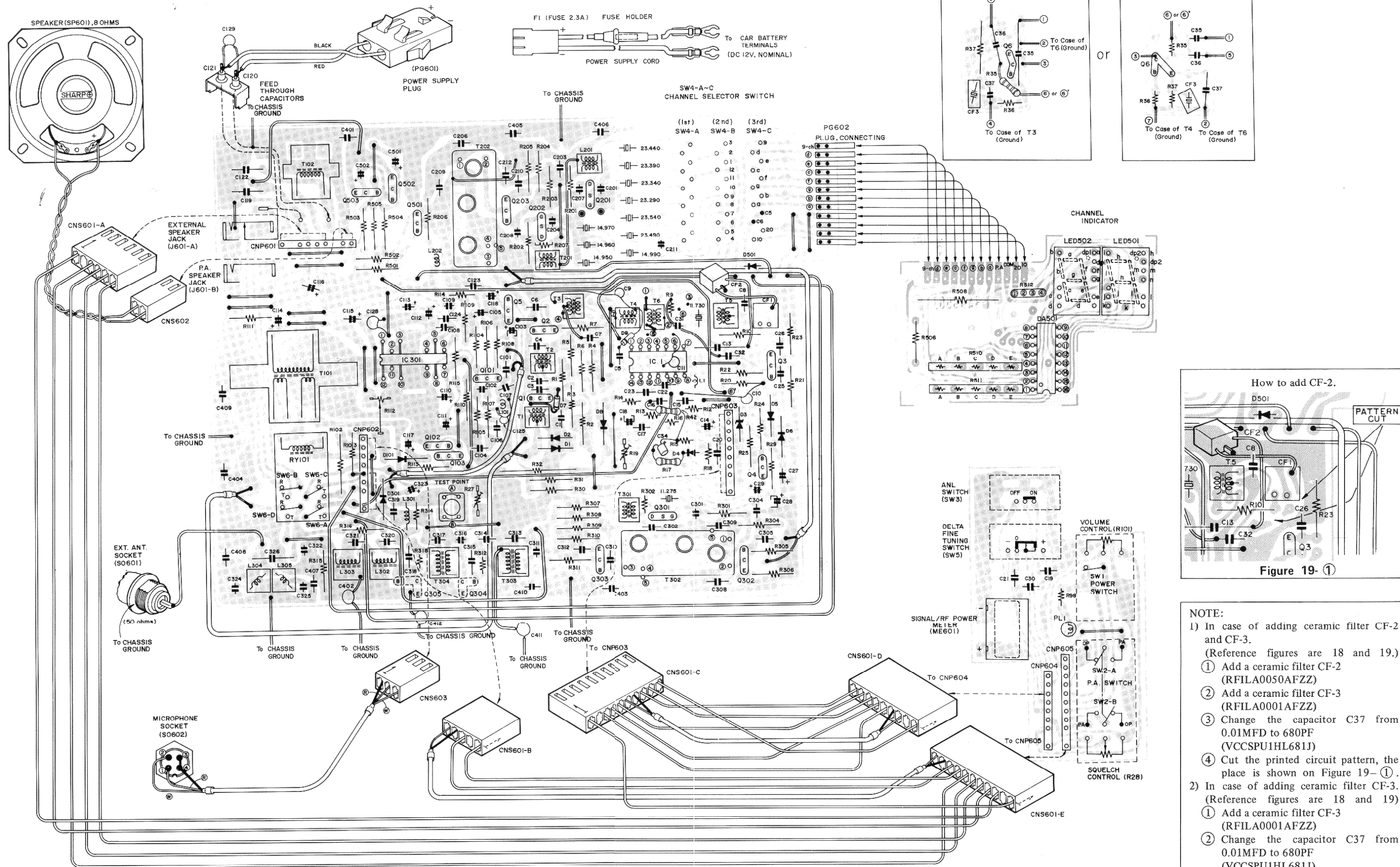
Figure 19 WIRING SIDE BOARD (P.W.B. NO. F0485AF-3)
