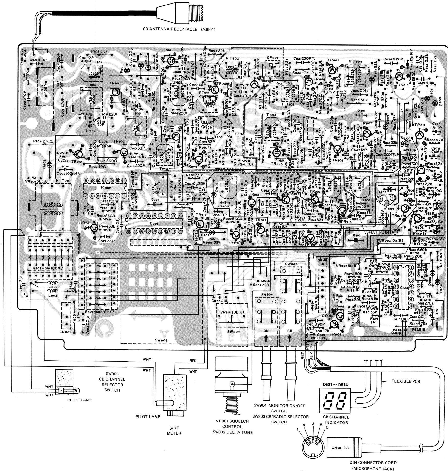
Figure 13. Printed Board - CB Block - 14T405
