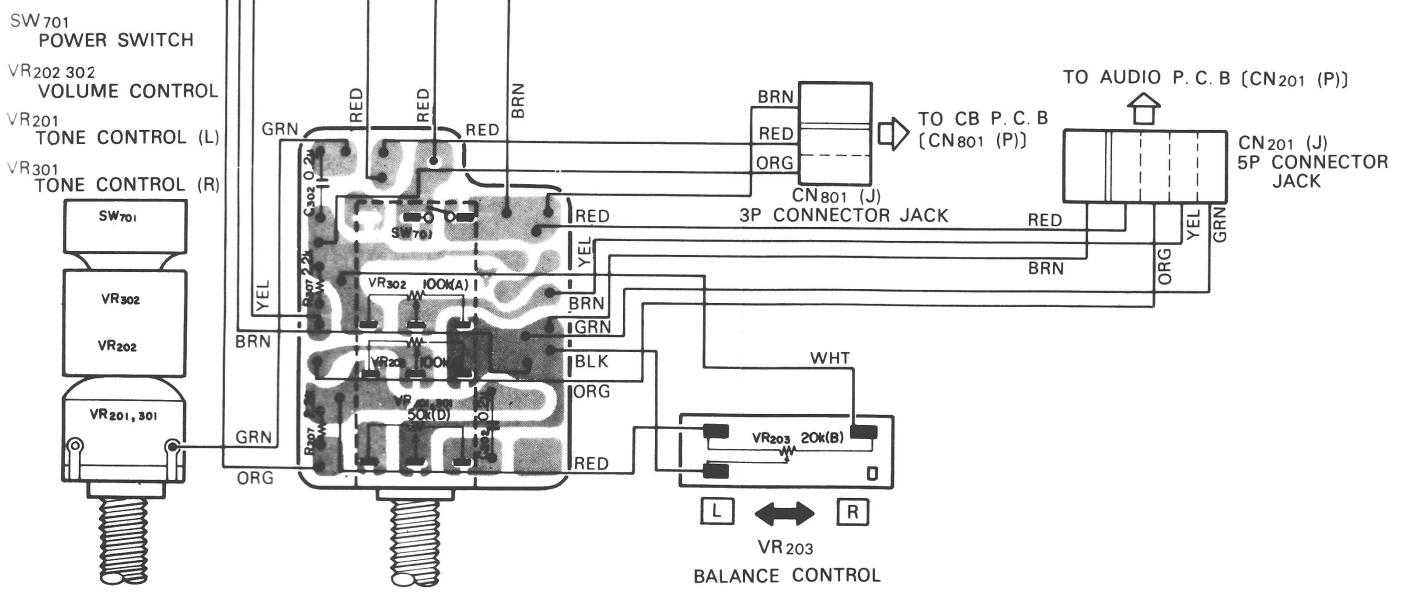
Figure 14. CB Transceiver, Power Block, and Controls, Wiring Diagram
