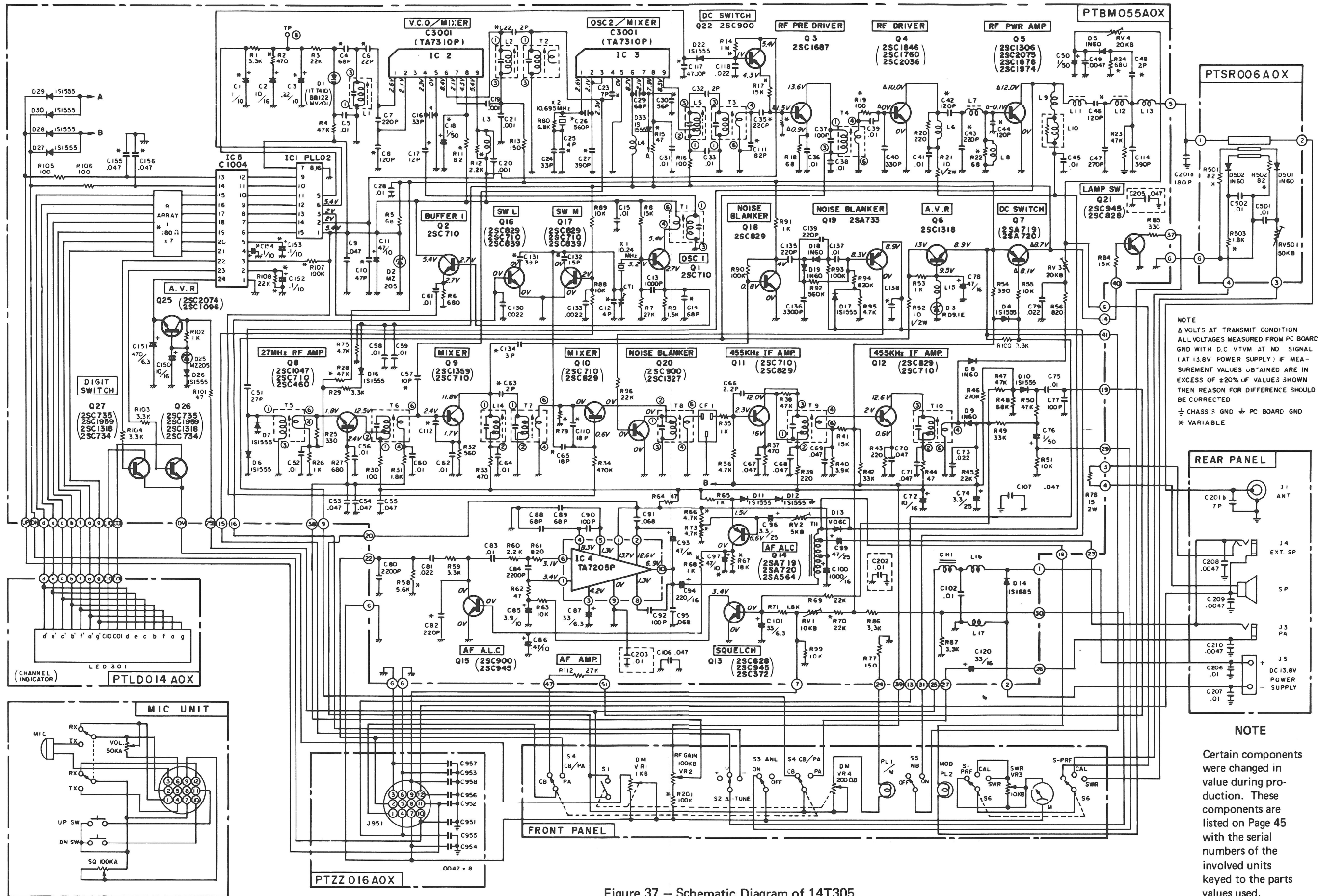
Figure 37 – Schematic Diagram of 14T305
