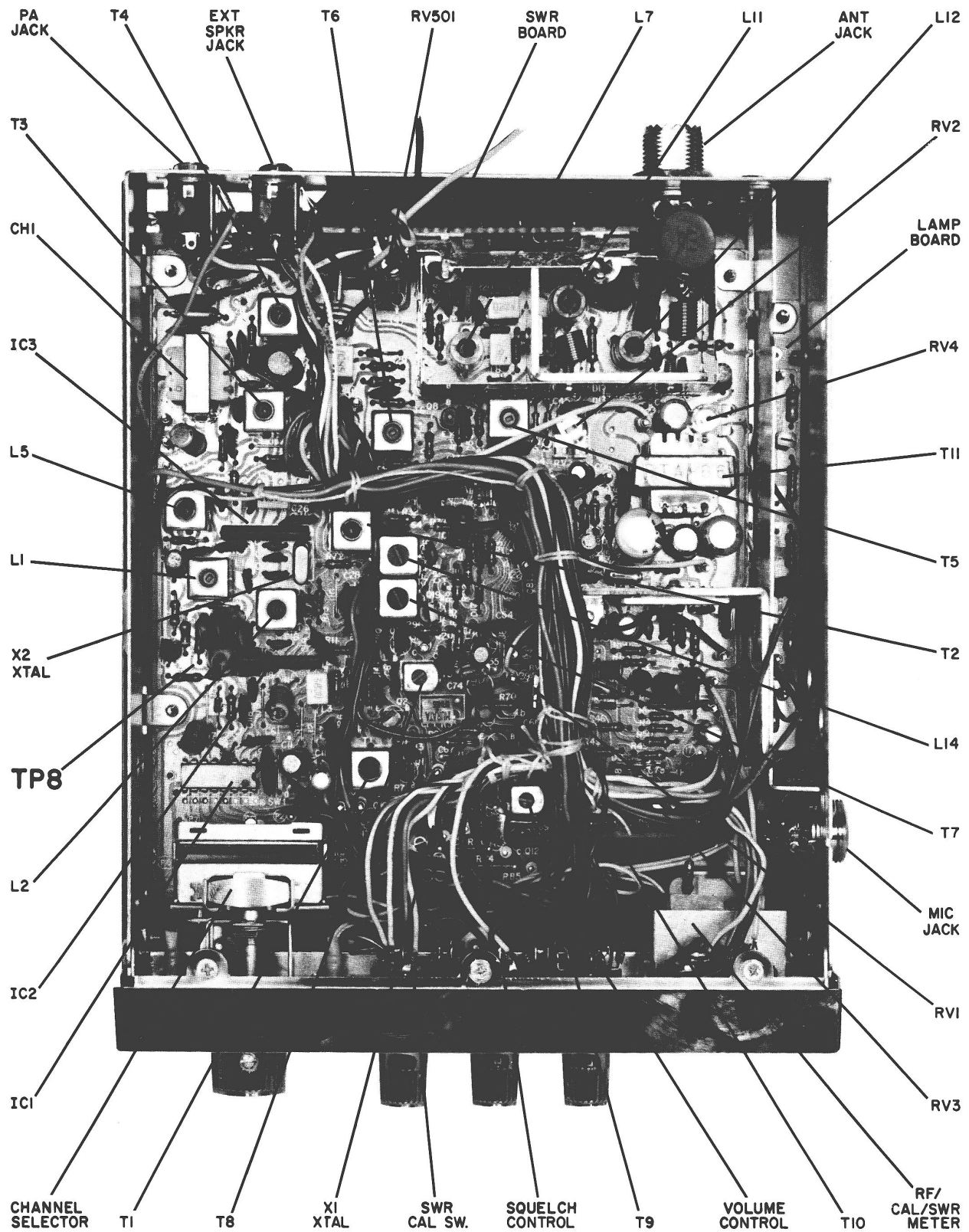
Figure 17 – Bottom (Component) View of Model 14T270
