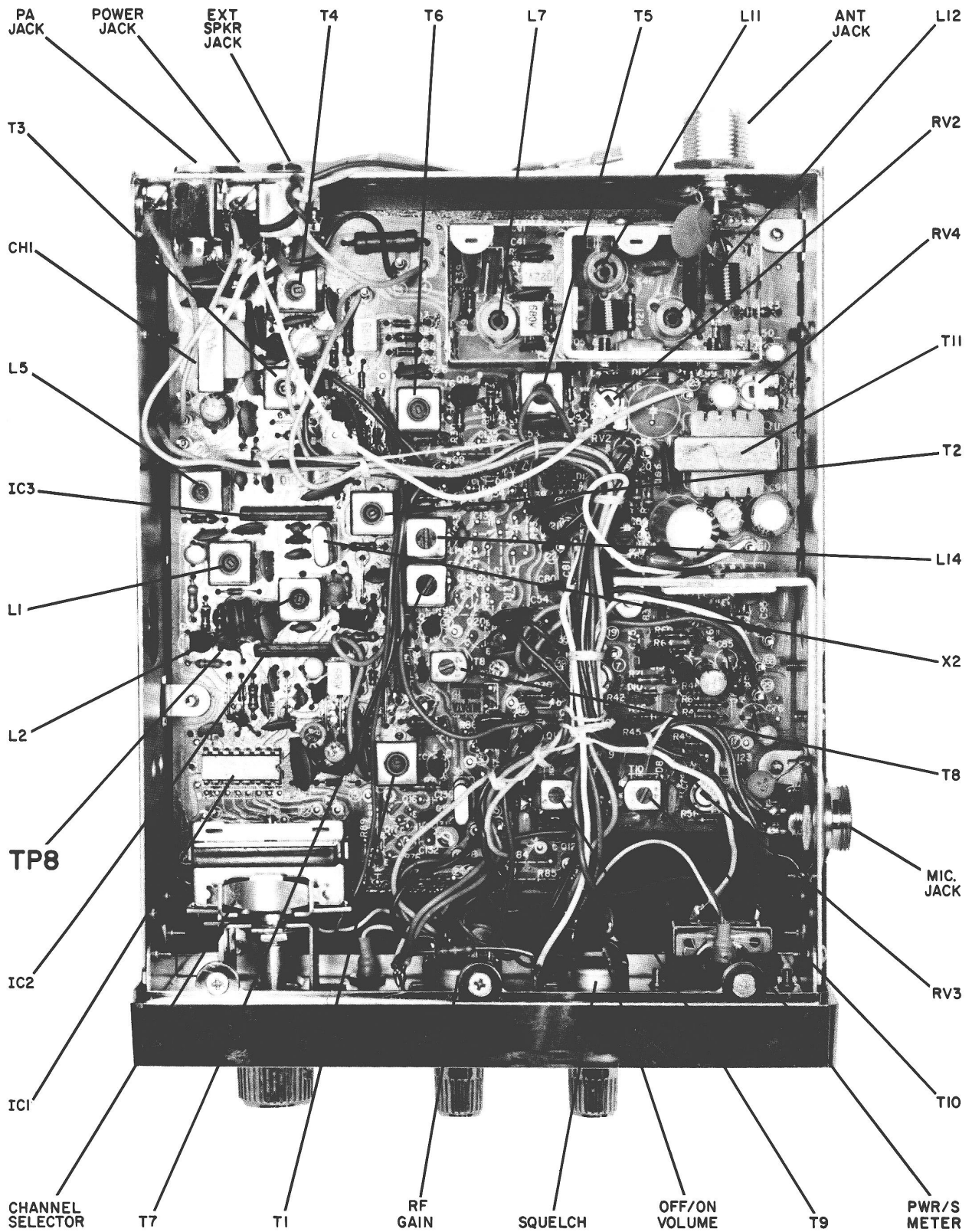
Figure 16 – Bottom (Component) View of Model 14T260
