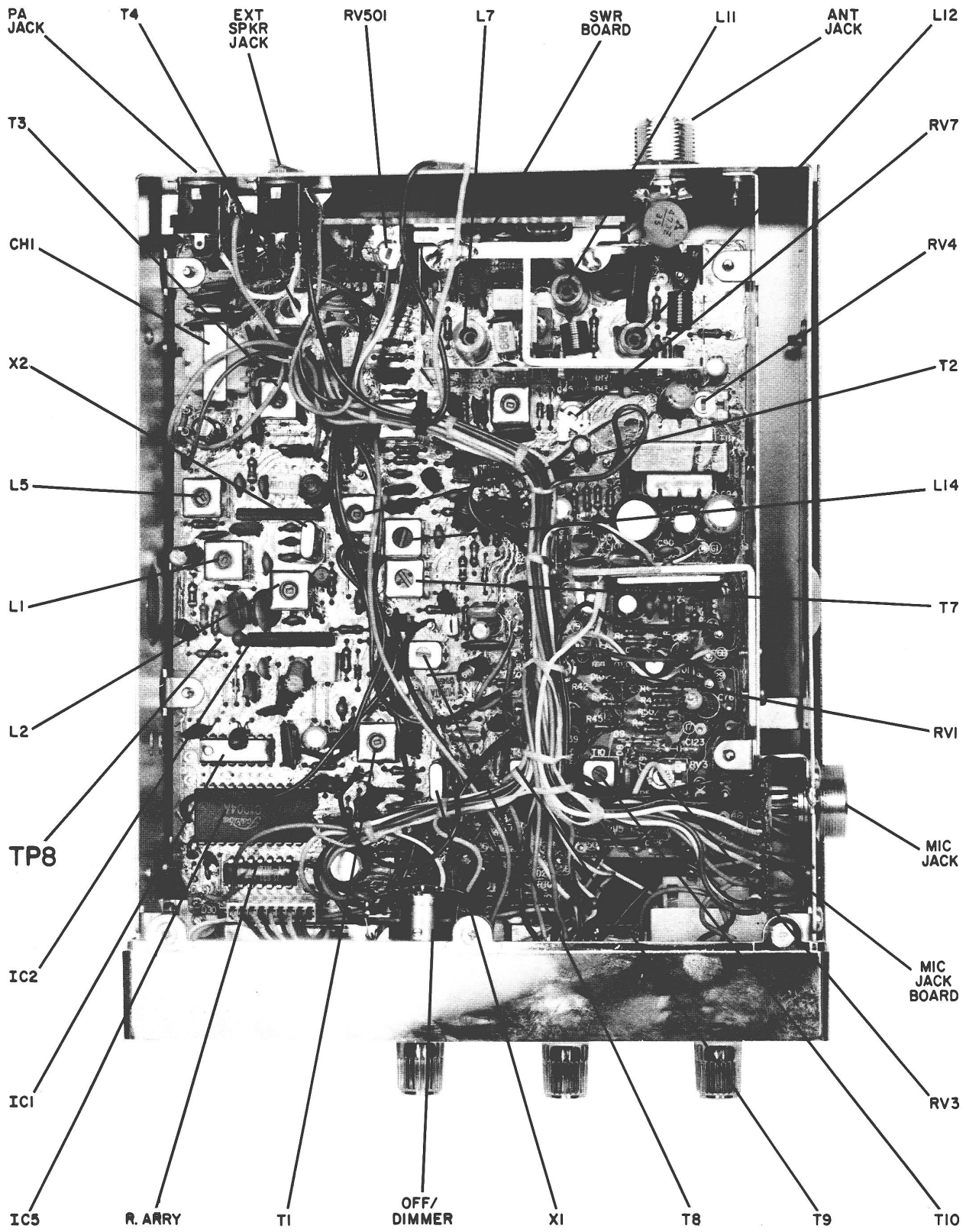
Figure 20 – Bottom (Component) View of Model 14T305
