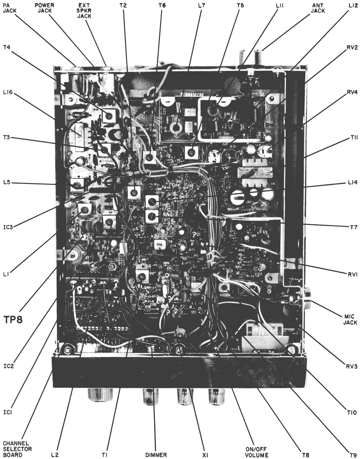
Figure 19 – Bottom (Component) View of Model 14T304
