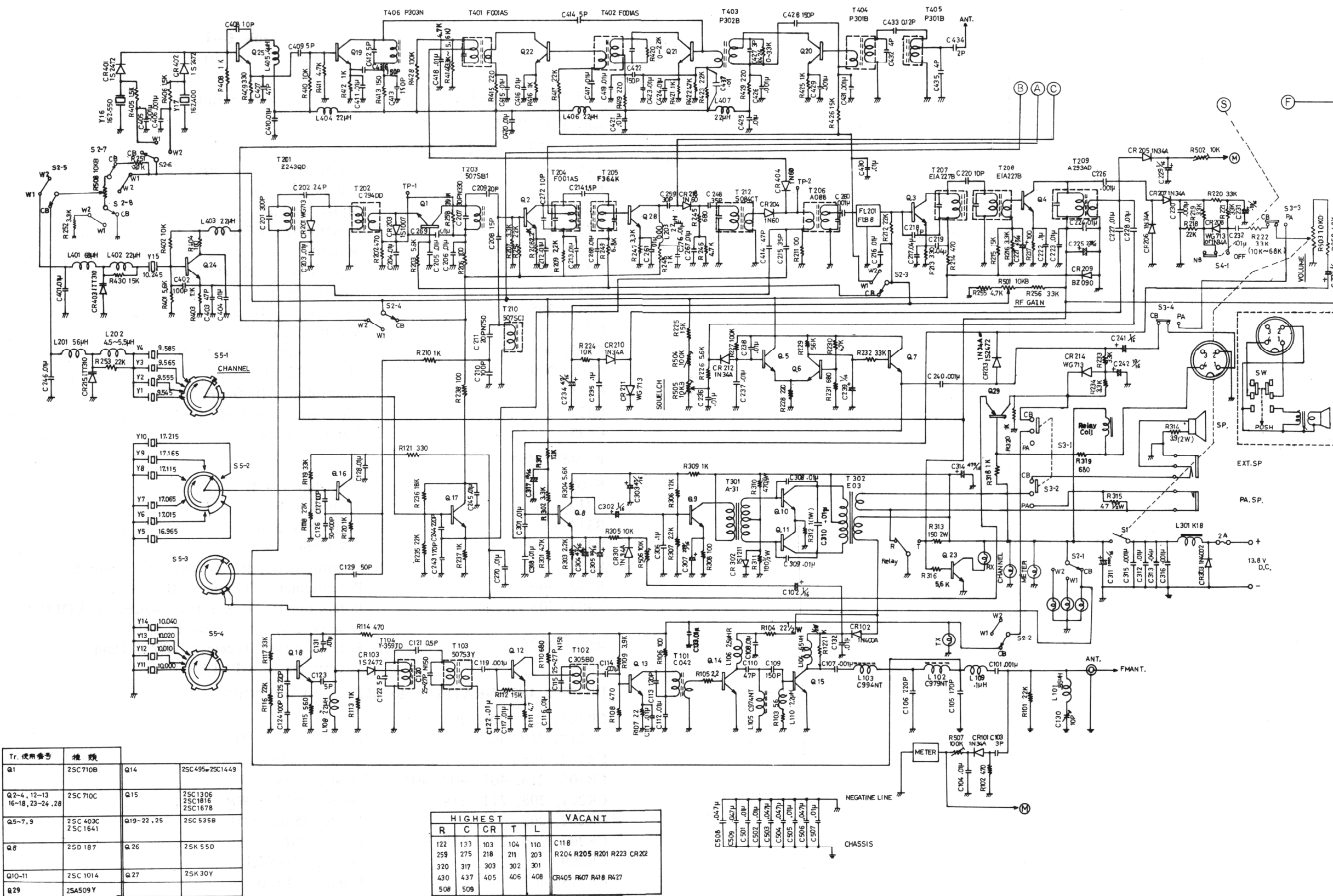
Figure 5-3 Schematic
