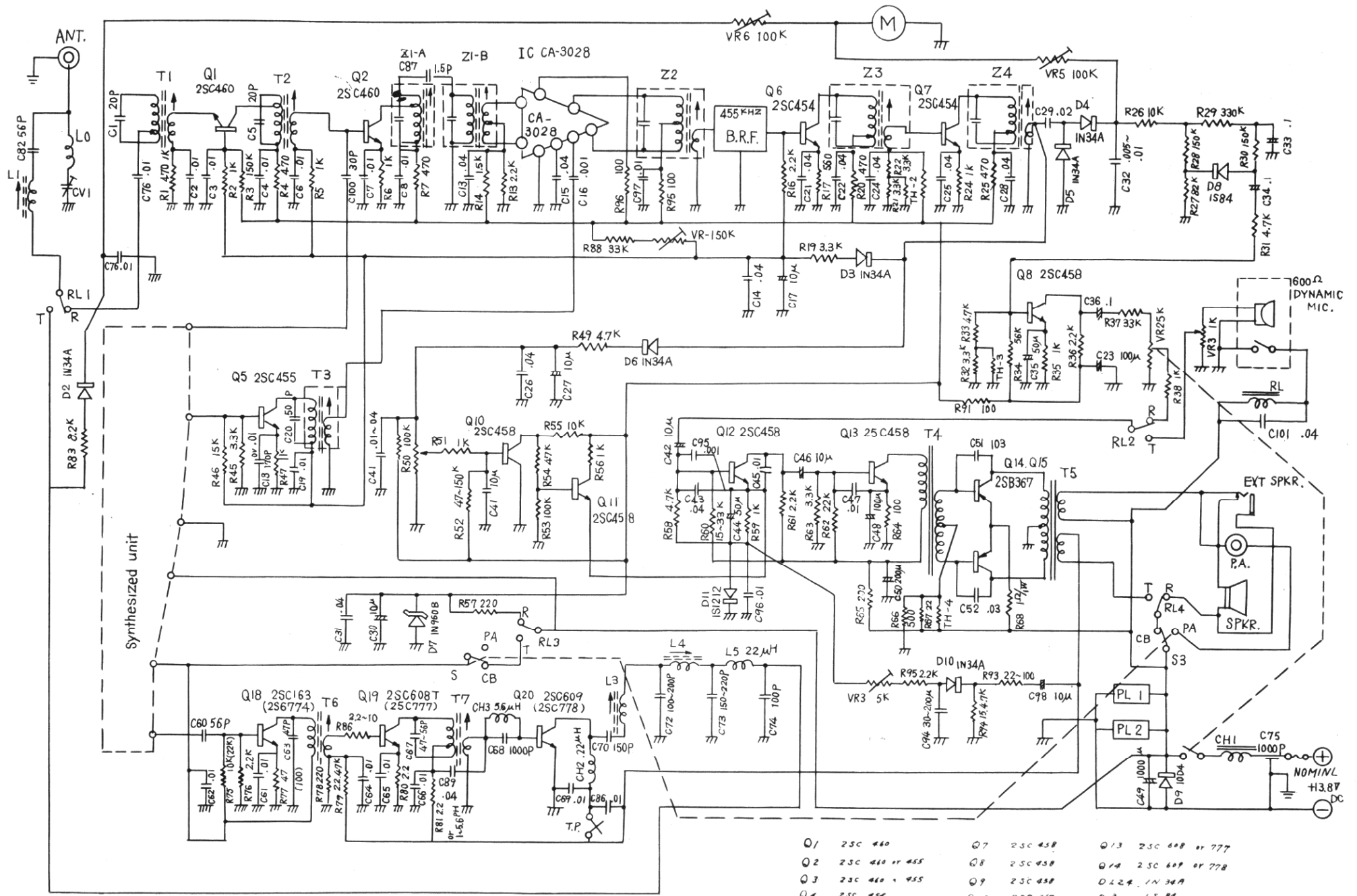
MODEL 13-870C SCHEMATIC DIAGRAM
