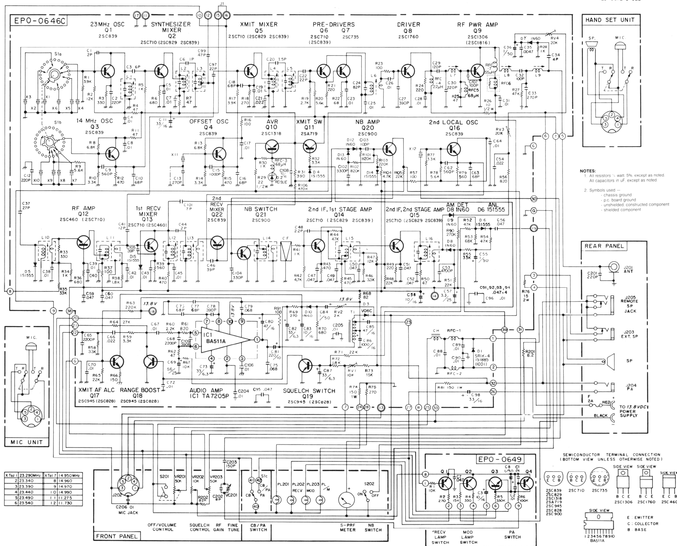
Figure 4-8. Schematic Diagram, 672B, Stage 3
