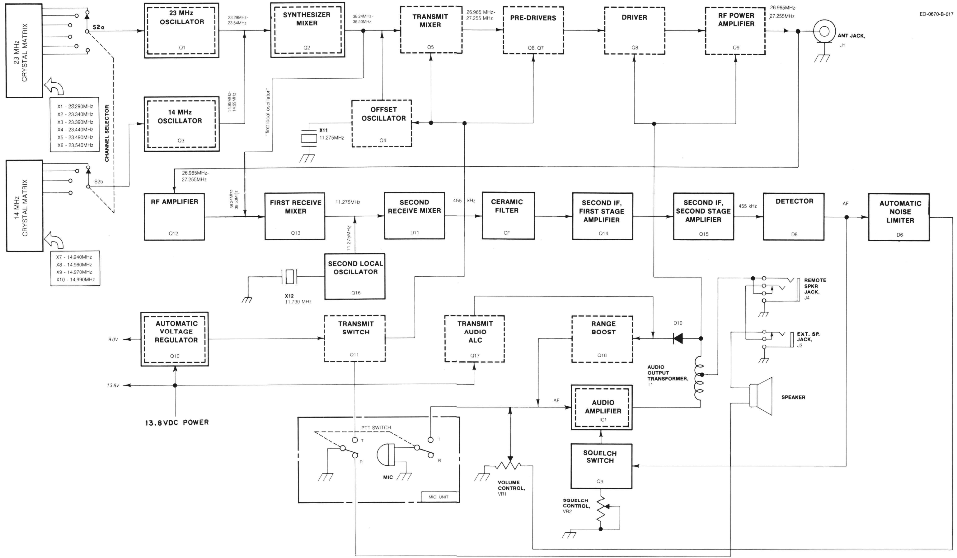
Figure 2-1. Block Diagram
