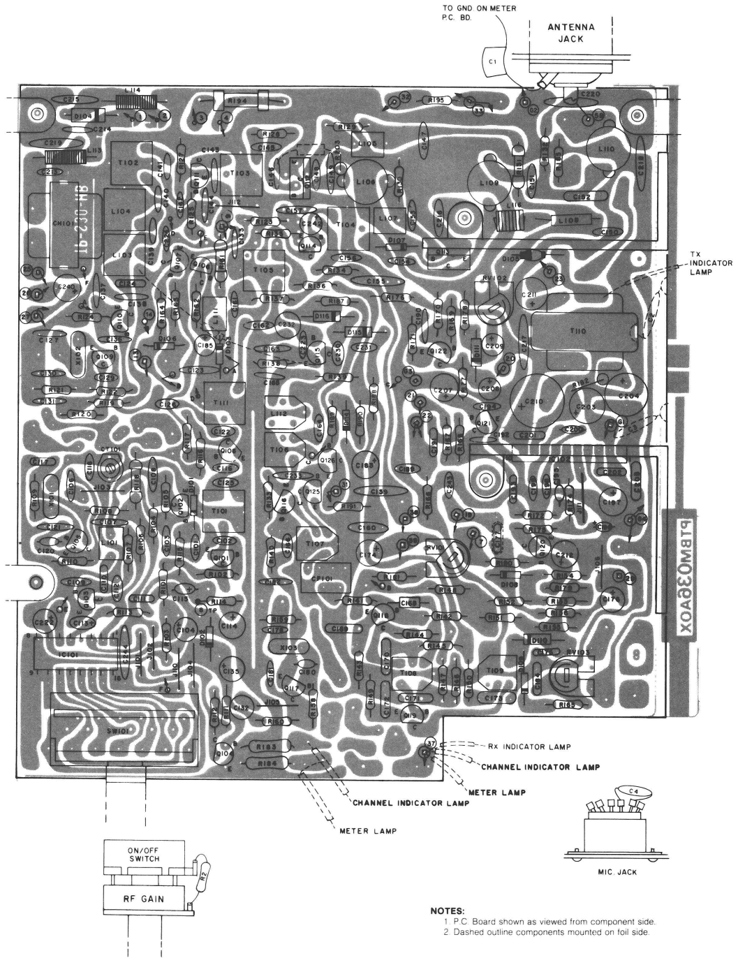
Figure 4-3. Main P.C. Component Outline. Model 2683
