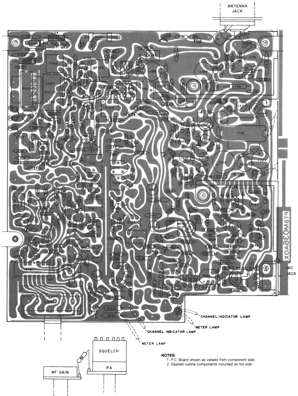
Figure 4-2. Component Outline, Model 2682
