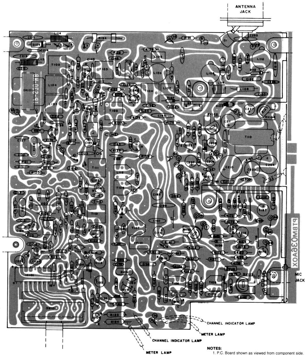
Figure 4-1. Component Outline, Model 2681
