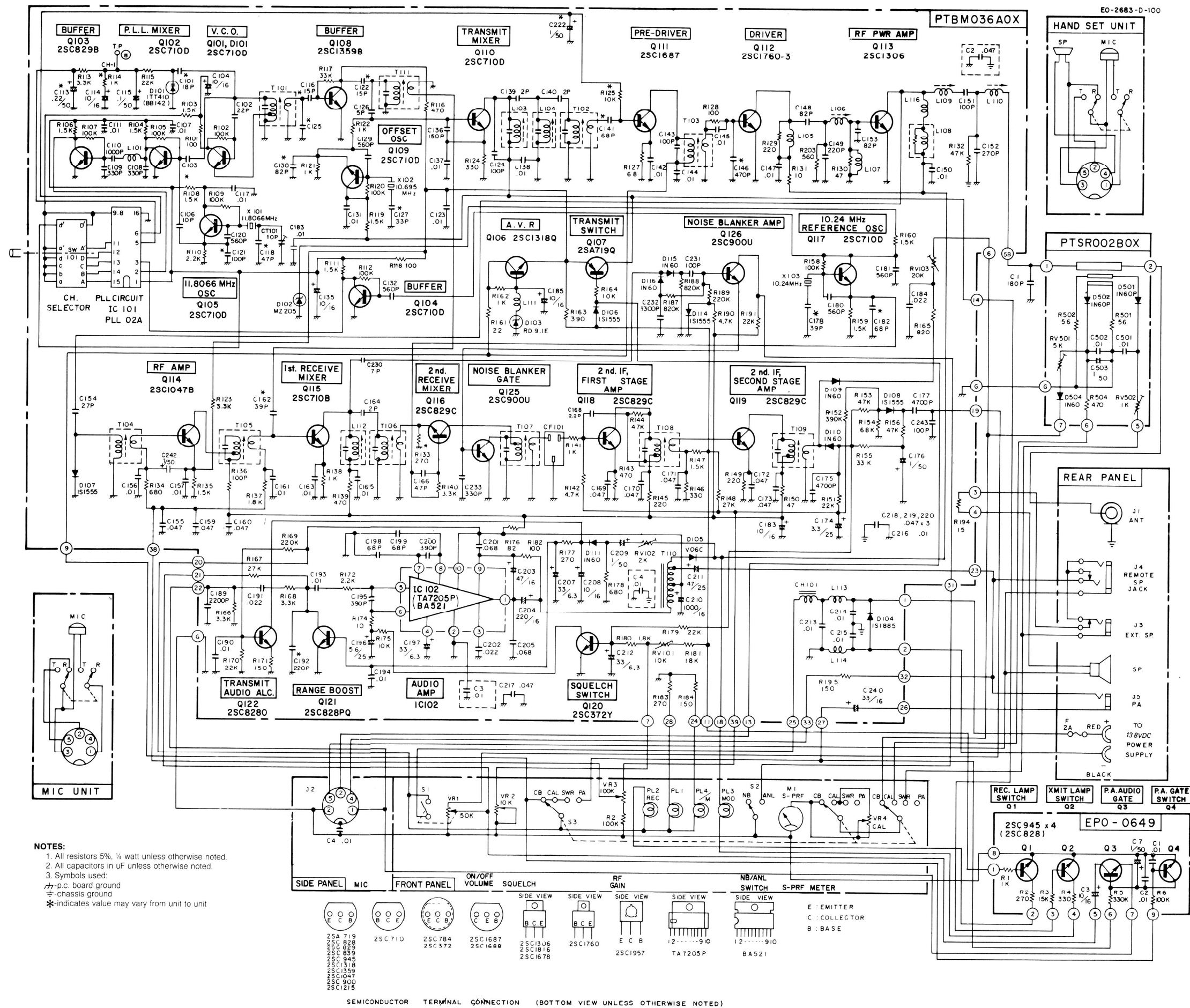
Figure 4-8. Schematic Diagram, Model 2683
