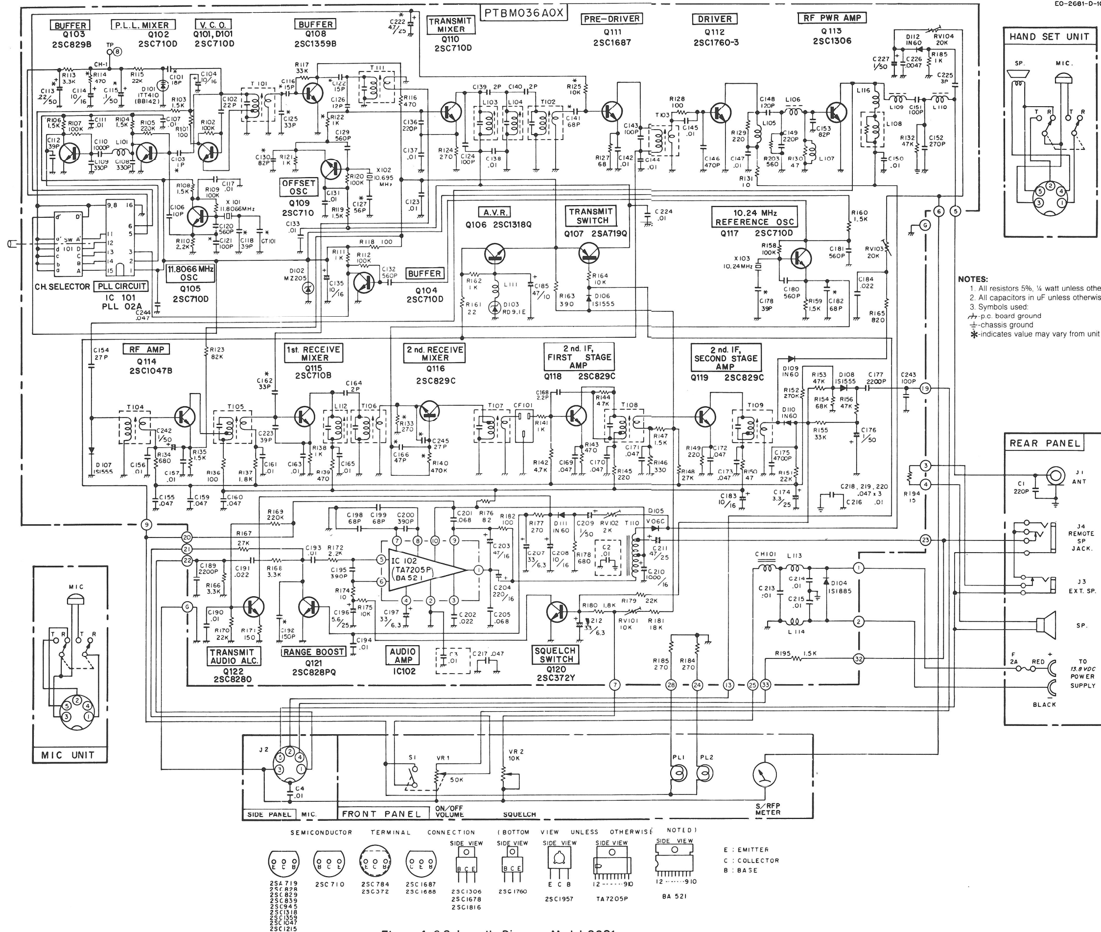
Figure 4-6. Schematic Diagram, Model 2681
