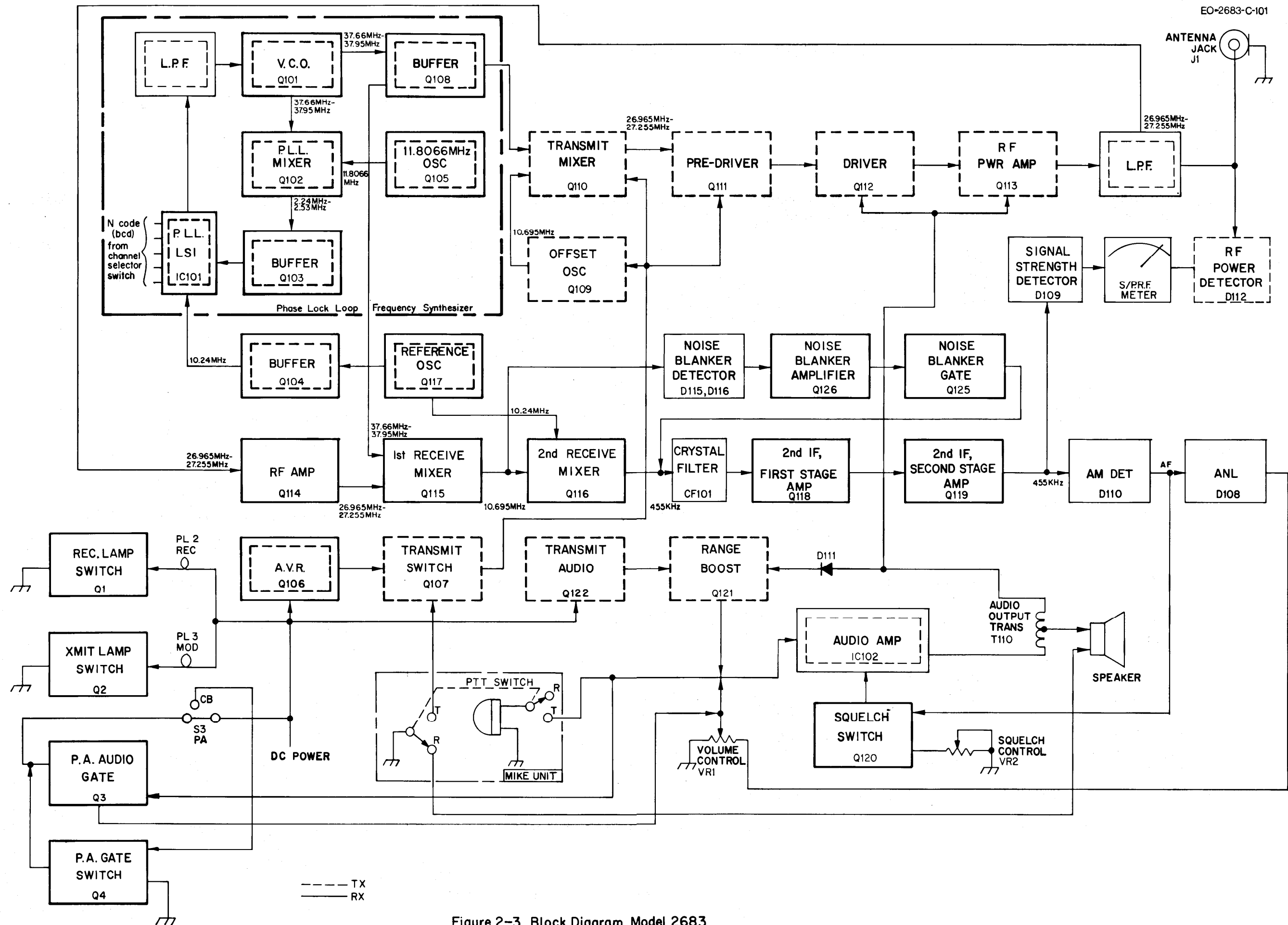
Figure 2-3. Block Diagram, Model 2683
