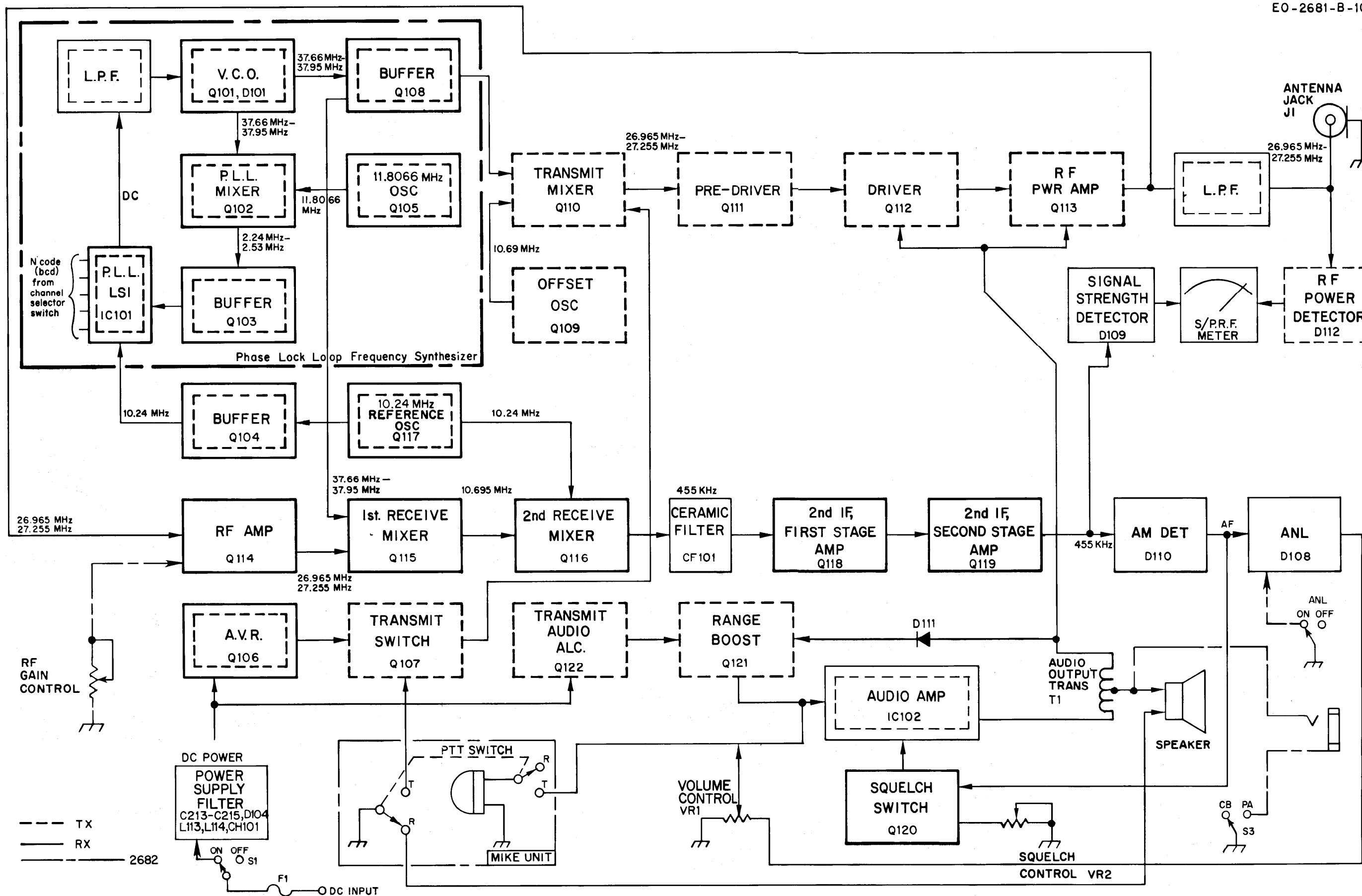
Figure 2-2. Block Diagram, Models 2681 & 2682
