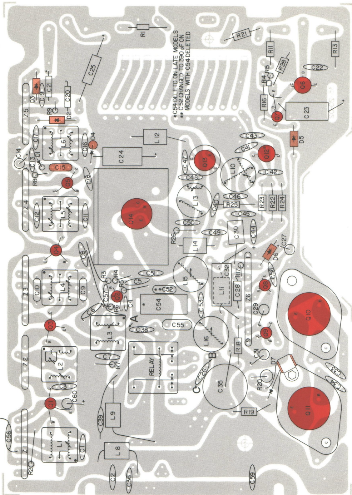
MESSENGER 100/110 PRINTED CIRCUIT BOARD (Top View)
