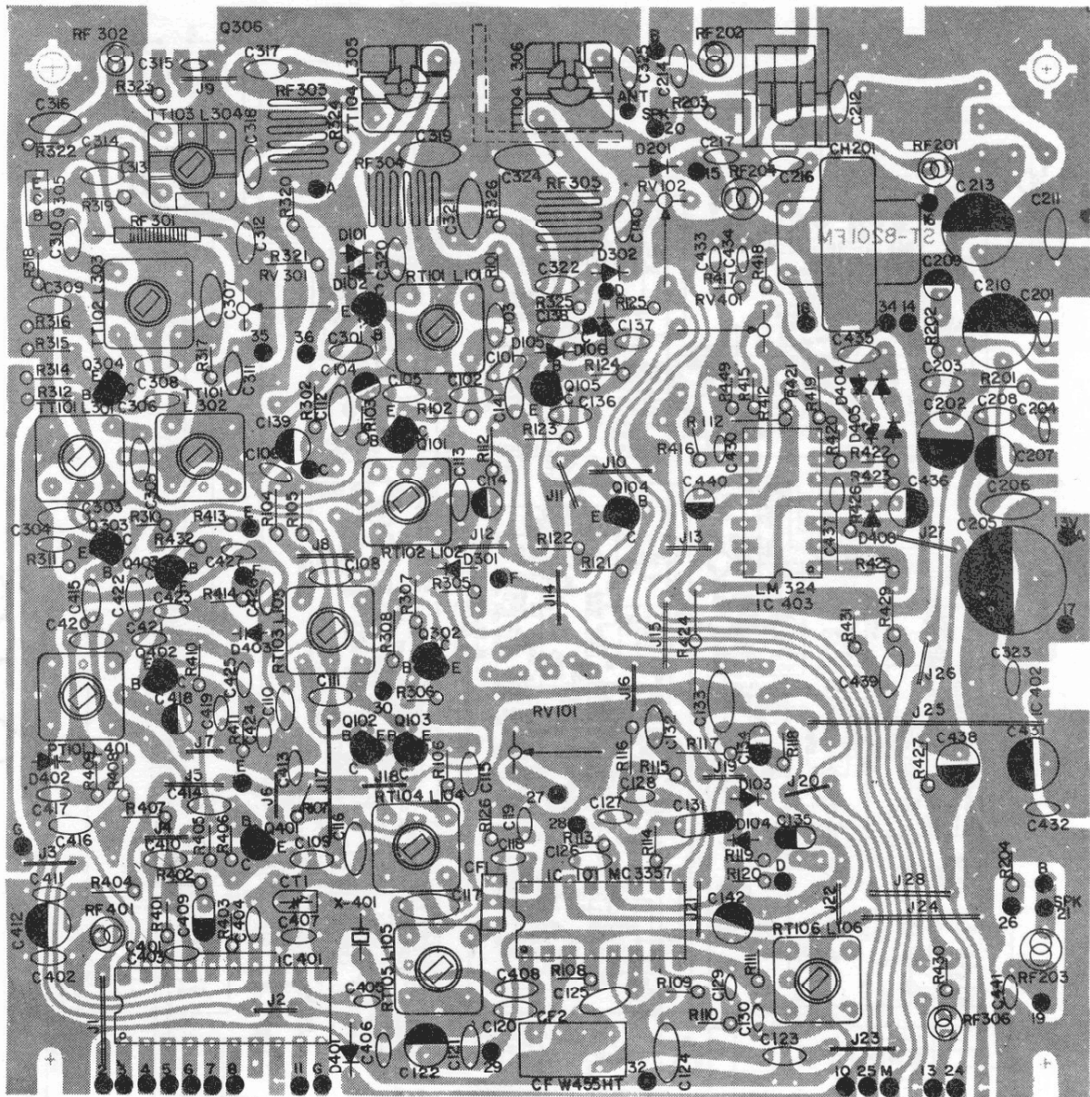
Component side
