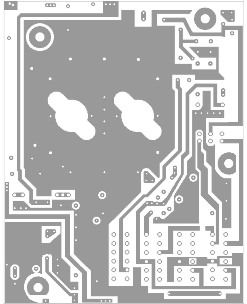
Board B Bottom View
