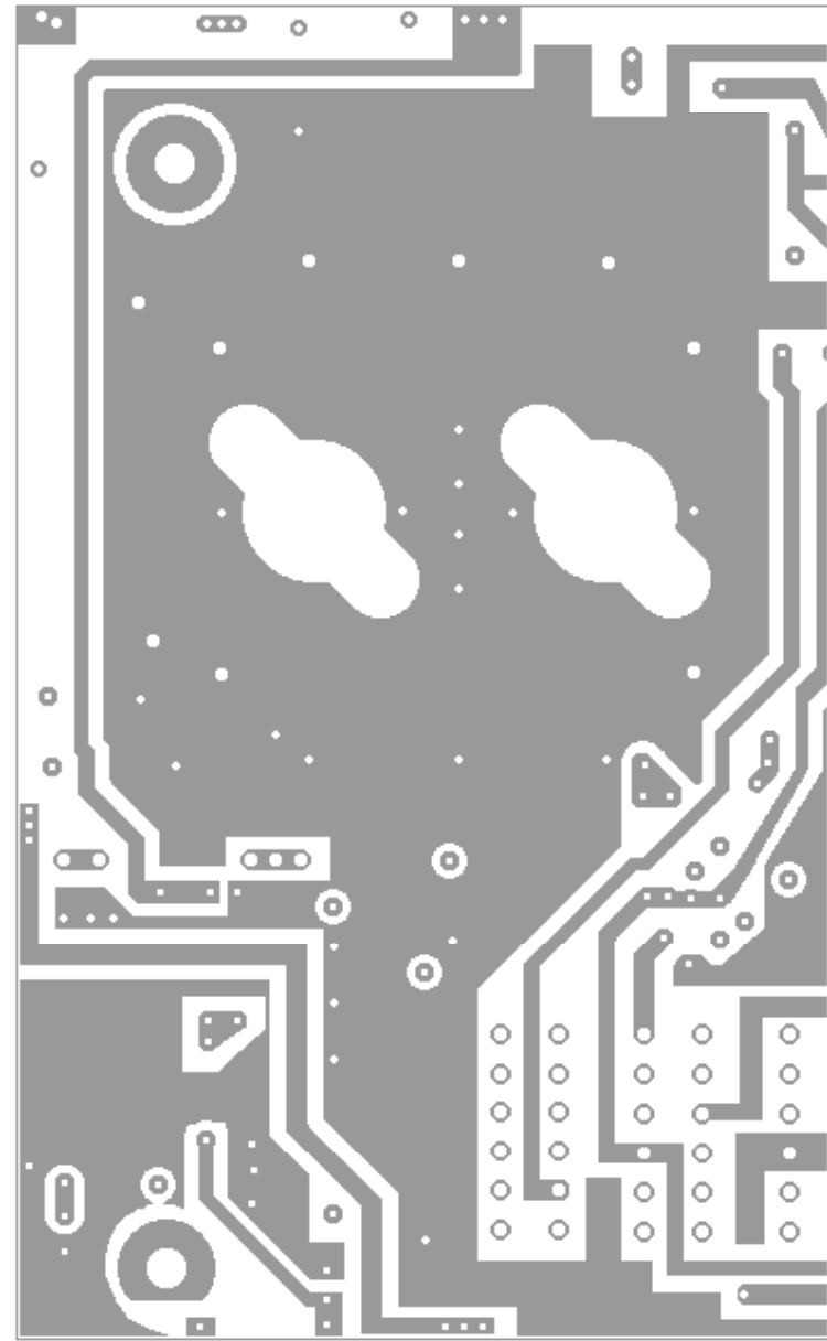
Board C Bottom View
