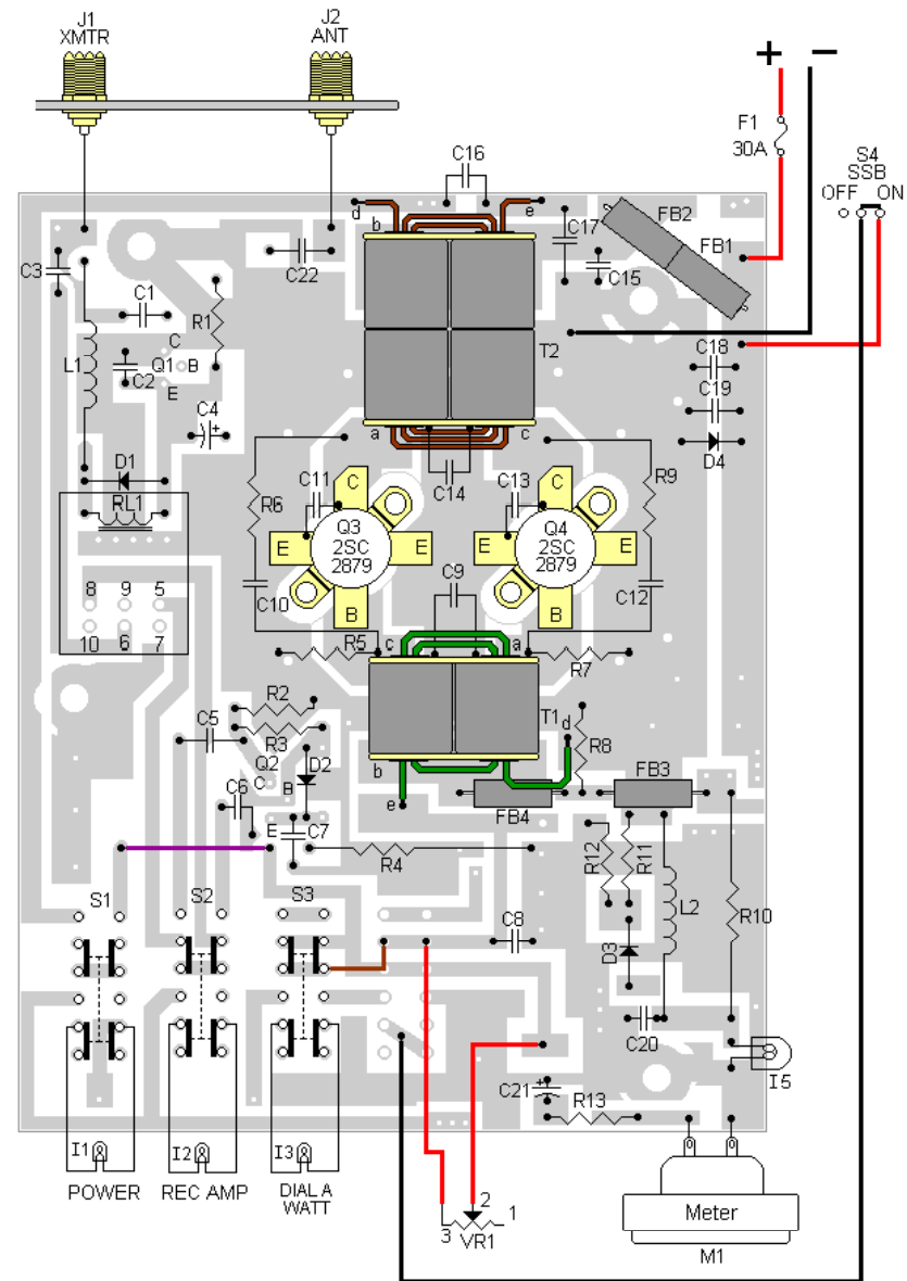
Texas Star DX 350 HDV Amp After Conversion CBTricks.com Rev # 1.6 Copyright © 2001, CBTricks.com All Rights Reserved Sep. 2001
