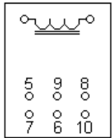
RL1 BOTTOM VIEW
