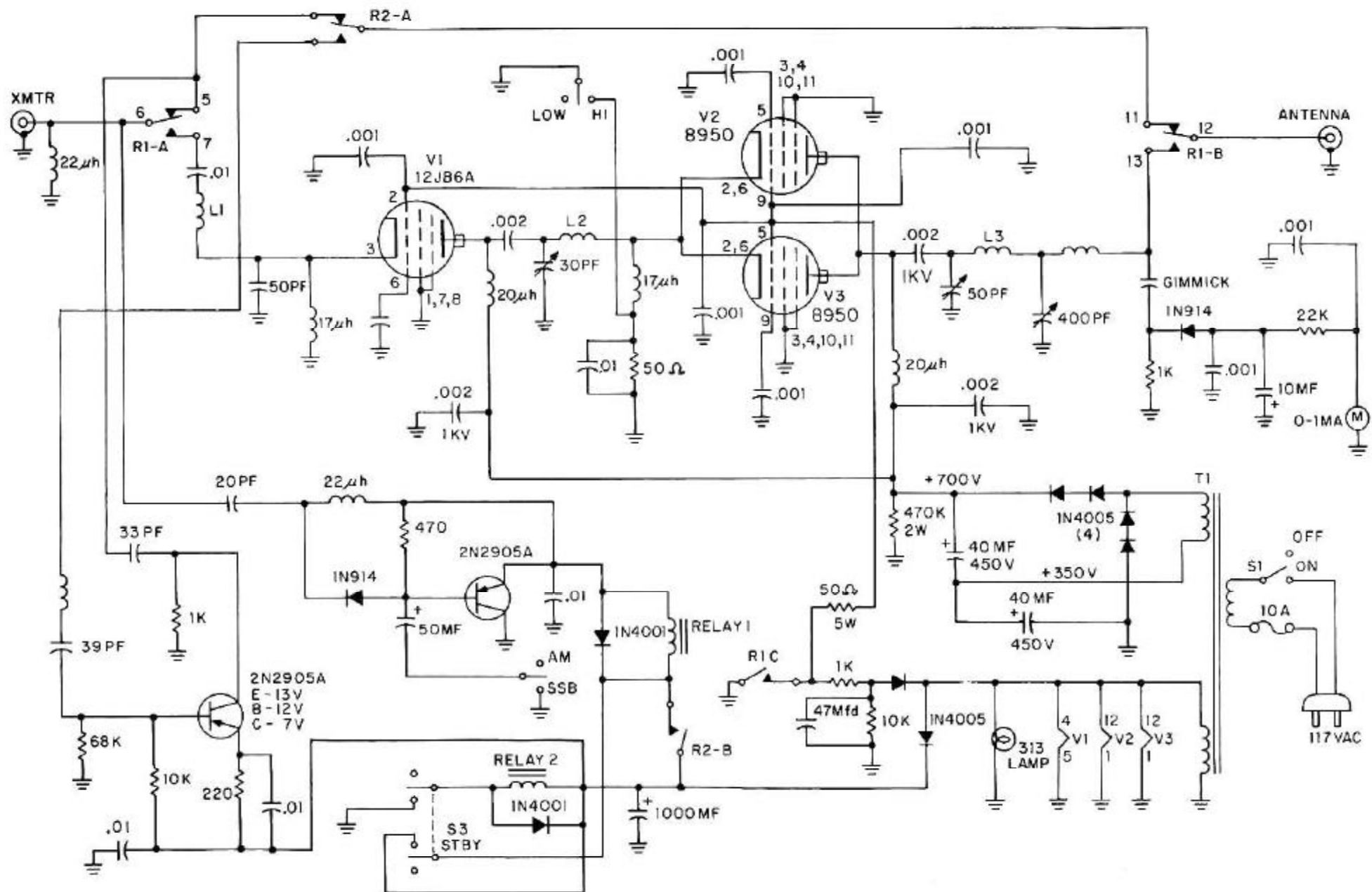
MODEL 221 BI-LINEAR AMPLIFIER
